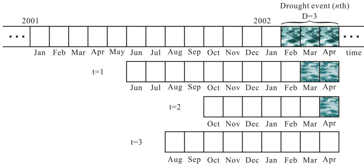
1 2 Figure. 3 The schematic diagram of determining the CPD.
