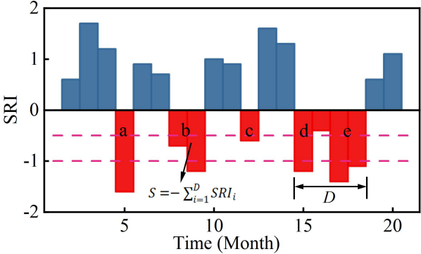
25 Figure. 2 Drought identification process and definition of drought characteristic variables.
