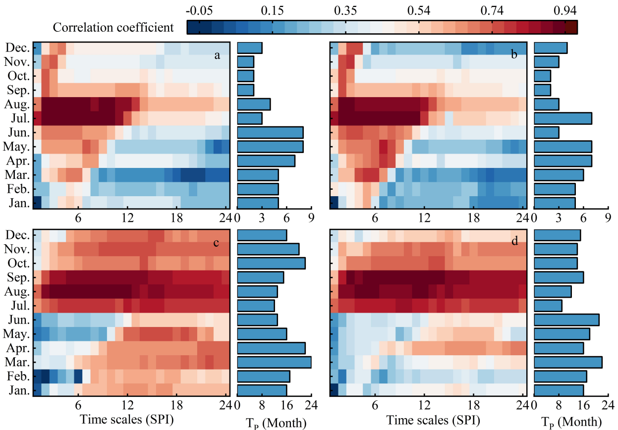
15 16 Figure. 8 The correlation between monthly SRI and multi-time scale SPI and the T_p in BKQ (a), DHF (b), SY (c) and XJWP (d).
