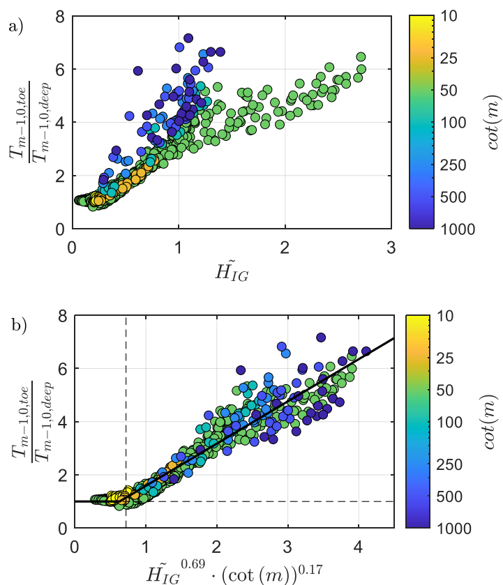
Figure B. 2 Numerically modelled relative spectral wave period as a function of a) \tilde{H}_{IG} alone; and b) \tilde{H}_{IG} and an additional foreshore-slope term. Solid line represents Equation 13. Dashed vertical line indicates h_{toe}/H_{m0,deep} = 1 and dashed horizontal line represents the deep-water limit where T_{m-1,0,toe}/T_{m-1,0,deep} \approx 1 .
