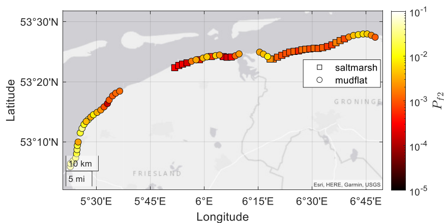
Figure 17: Influence of raised bed levels due to saltmarshes on the spatial variation in the probability of dike failure by wave overtopping for scenario 2: SS + IG waves ( P_{f2} ) across the wider Dutch Wadden Sea area for dikes with identical crest heights ( z_c = 6\text{m} ) and dike slopes ( \cot(\alpha) = 7 ).
