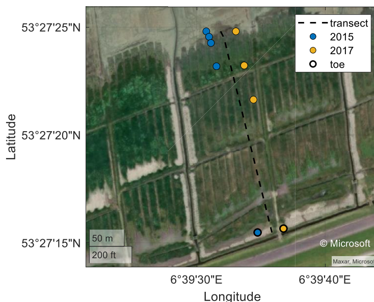
Figure 5 Wave gauges locations for the January 2015 and January 2017 field campaigns at Uithuizerwad (corresponding to the star in Figure 1).
