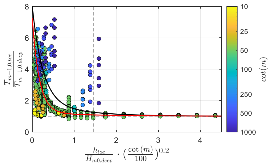
Figure B. 1 Numerically modelled relative spectral wave period as a function of relative water depth and foreshore slope, following Hofland et al. (2017). Black and red lines represent Equations B.1 and B.2, respectively.
