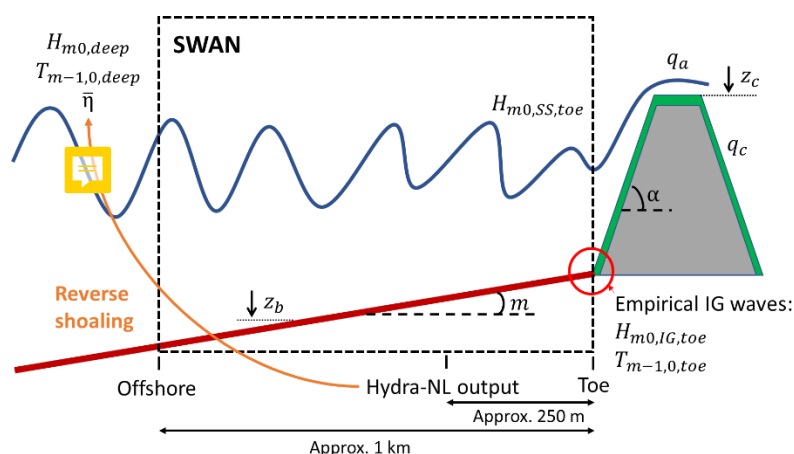
Figure 3: Schematic representation of the dike-foreshore system, showing the areas where key parameters and tools are applied. These parameters and tools are introduced throughout Section 2.2.
