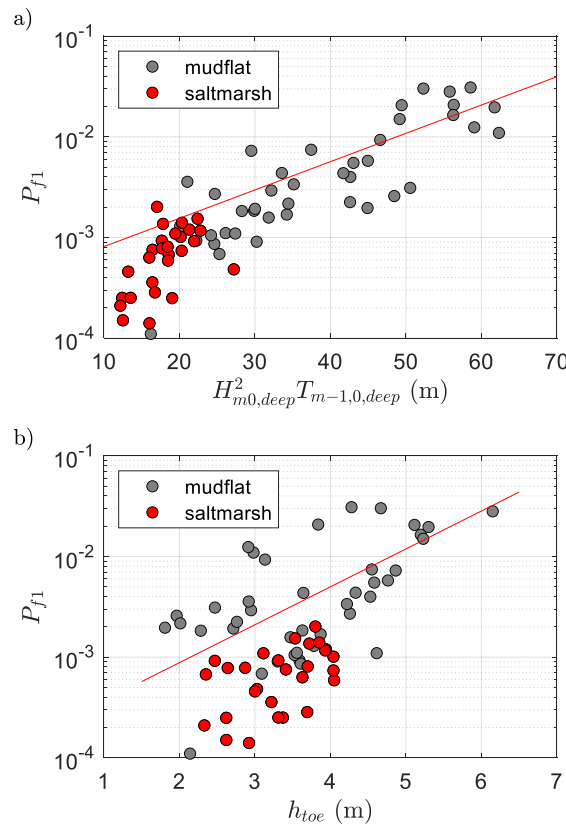
Figure 13: Relationship between probability of failure for scenario 1 (SS) and: a) an offshore forcing parameter; and b) the water depth at the dike toe ( h_{toe} ), across the wider Dutch Wadden Sea area. Lines indicate best-fit through the data.
