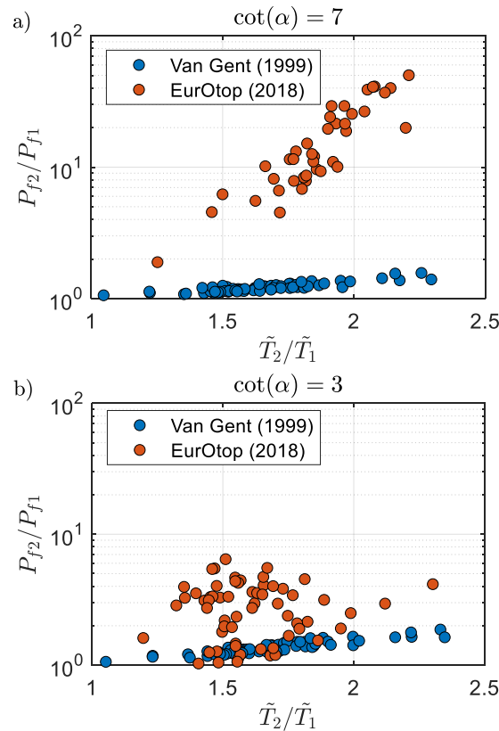
Figure 15: Relationship between the change in probability of failure due to IG waves ( P_{f2}/P_{f1} ) and the increase in relative spectral wave period at the toe ( \tilde{T}_2/\tilde{T}_1 ) calculated using the original Van Gent (1999) and EurOtop (2018) approaches for the actual overtopping discharge for a) \cot(\alpha) = 7 and b) \cot(\alpha) = 3 . Note that cases with wave steepness at the toe < 0.01 were excluded from the EurOtop (2018) calculations since the equivalent slope concept could not be applied (Section 4.2).
