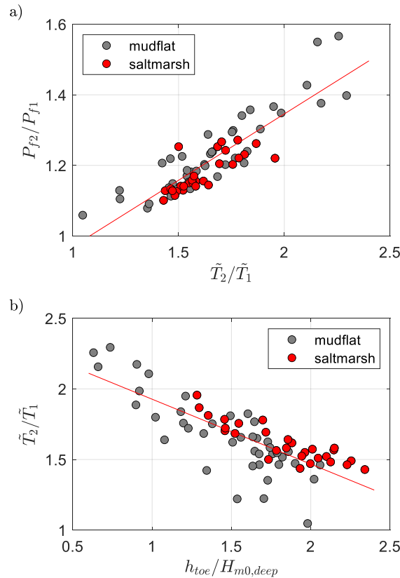
Figure 14: a) Relationship between the change in probability of failure due to IG waves ( P_{f2}/P_{f1} ) and the increase in relative spectral wave period at the toe ( \tilde{T}_2/\tilde{T}_1 ); and b) relationship between \tilde{T}_2/\tilde{T}_1 and the relative water depth ( h_{toe}/H_{m0,deep} ), across the wider Wadden area. Note that \tilde{T} is a stand-in for T_{m-1,0,toe}/T_{m-1,0,deep} . Subscripts 1 and 2 refer to scenarios 1 and 2, respectively.
