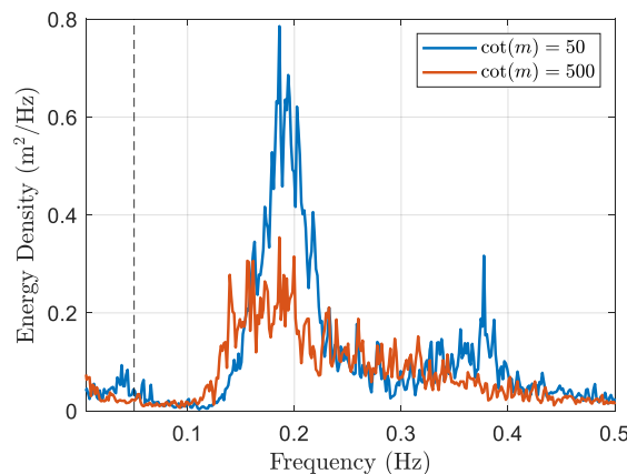
545 Figure 16: Results of XBeach numerical simulations showing wave spectra at the dike toe for a 1:50 and 1:500 foreshore slope, under the same offshore forcing conditions ( H_{m0,deep} = 1 m, T_{m-1,0,deep} = 4.54 s and h_{toe} = 1 m). Dashed vertical line indicates the frequency separating IG and SS wave motions.
