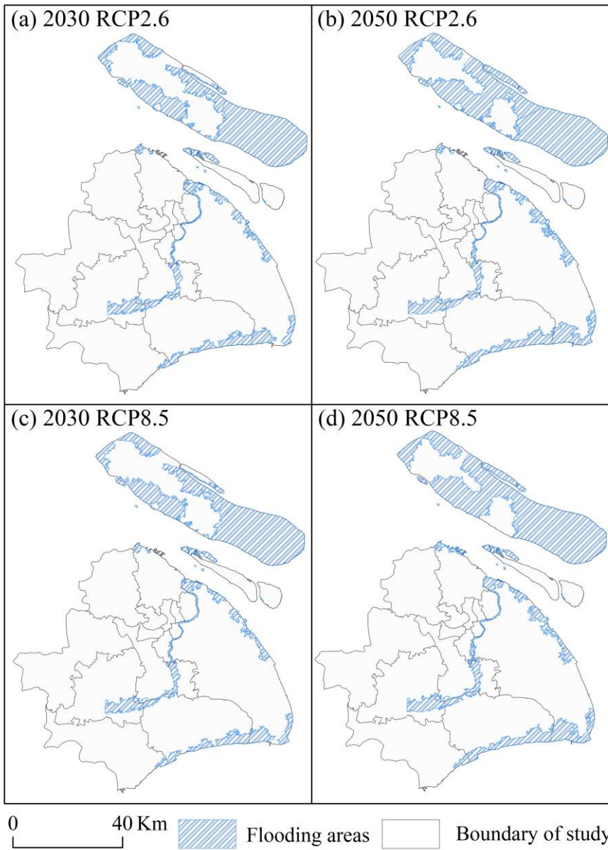
11 Figure S1: The flood inundation in RCP2.6 and RCP8.5 scenarios.
