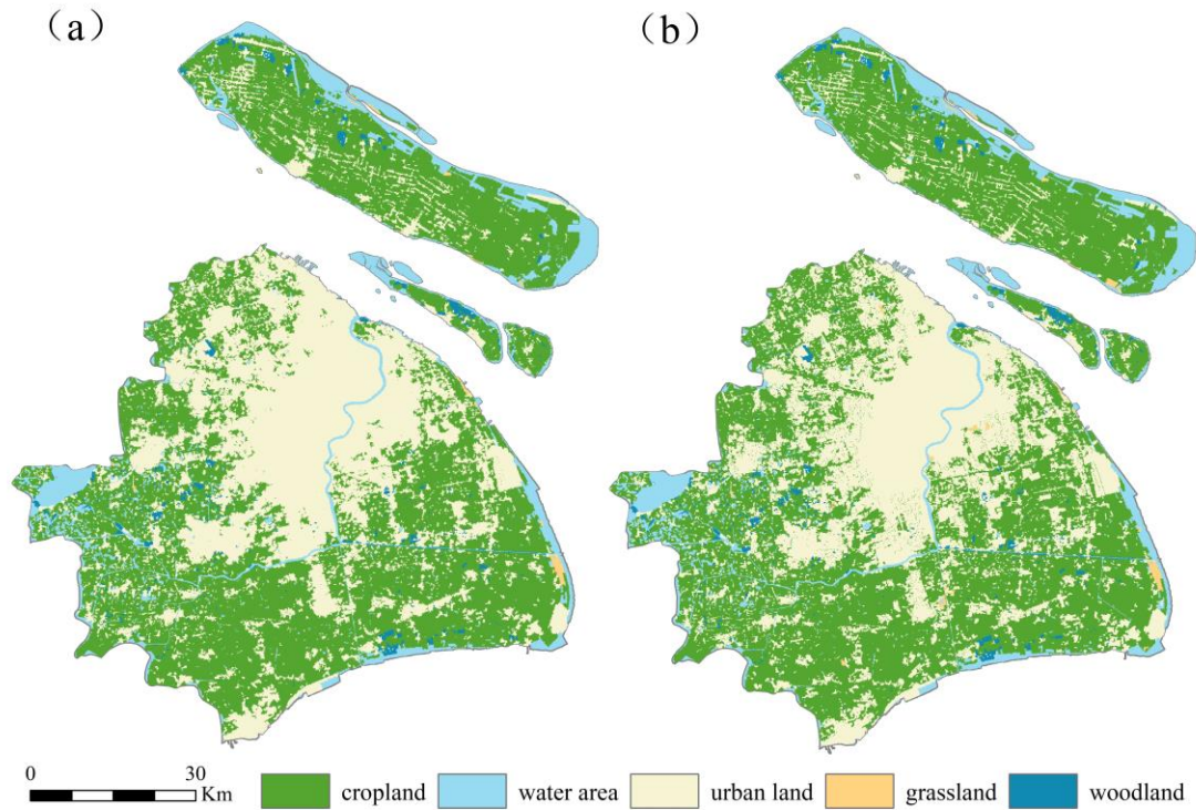
219 220 Figure 3: Comparing the simulation results of Shanghai urban expansion with the actual situation, (a) simulation result in 2015; (b) 221 actual land use in 2015.
