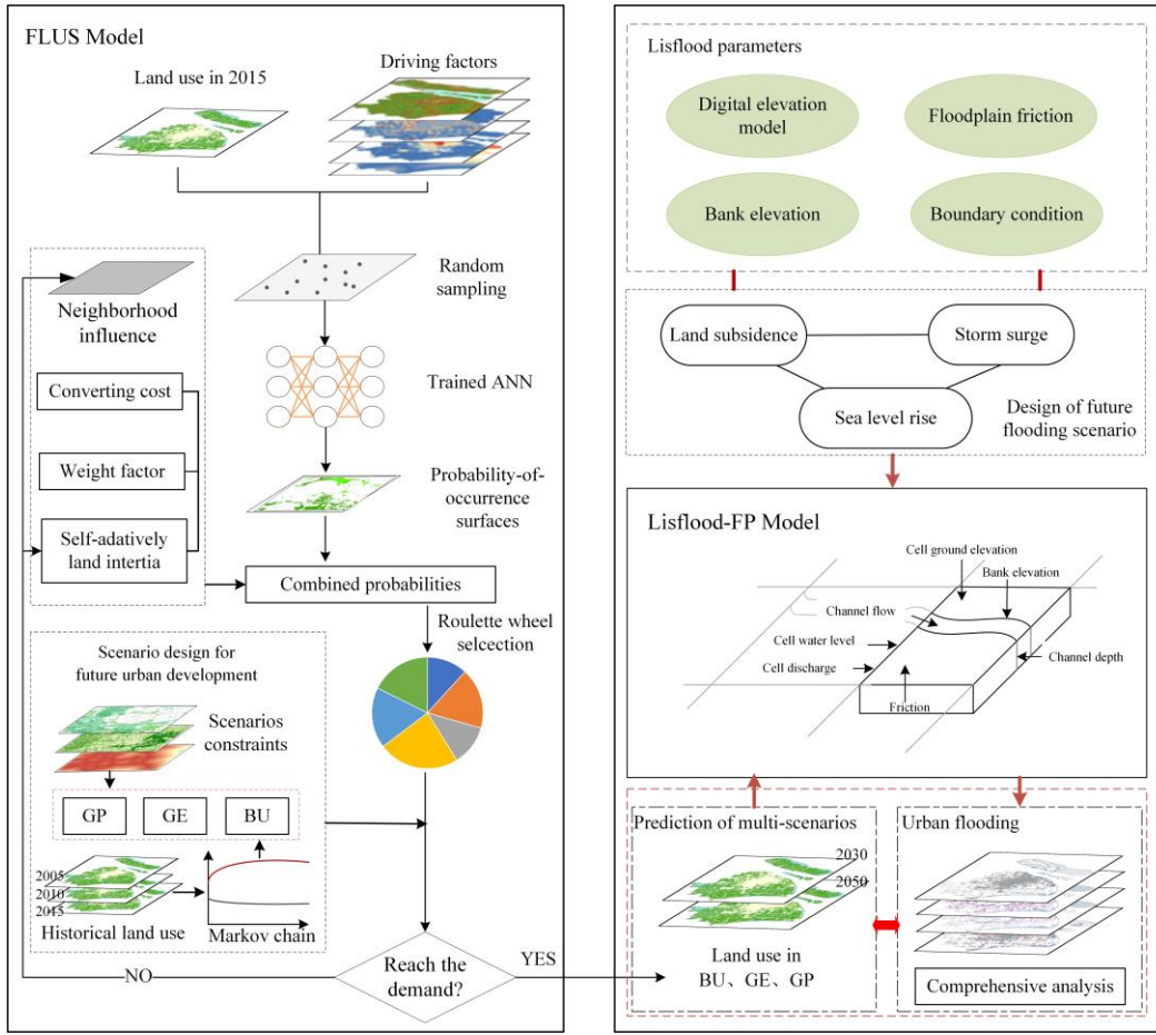
137 138 Figure 2: The overall flow chart of research.
