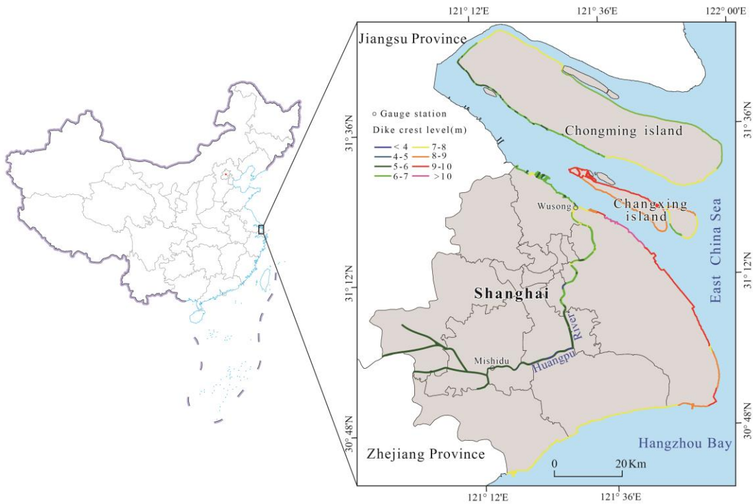
89 Figure 1: Location map of the study area. The main inland rivers in Shanghai flow into the East China Sea through the Huangpu 90 River. The line with coloured vectors in the figure indicates the different dike crest level in Shanghai.
