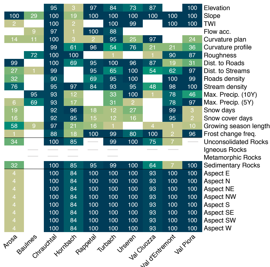
Figure 5. Heat-map displaying the inclusion rate of variables for all 10 sites. The numbers indicate how often variables were selected for the models out of 100 estimates. Note that not all geological rock classes are present at all sites (grey line). Darker colors show variables selected more often. White boxes indicate which variables were never selected for the models.
