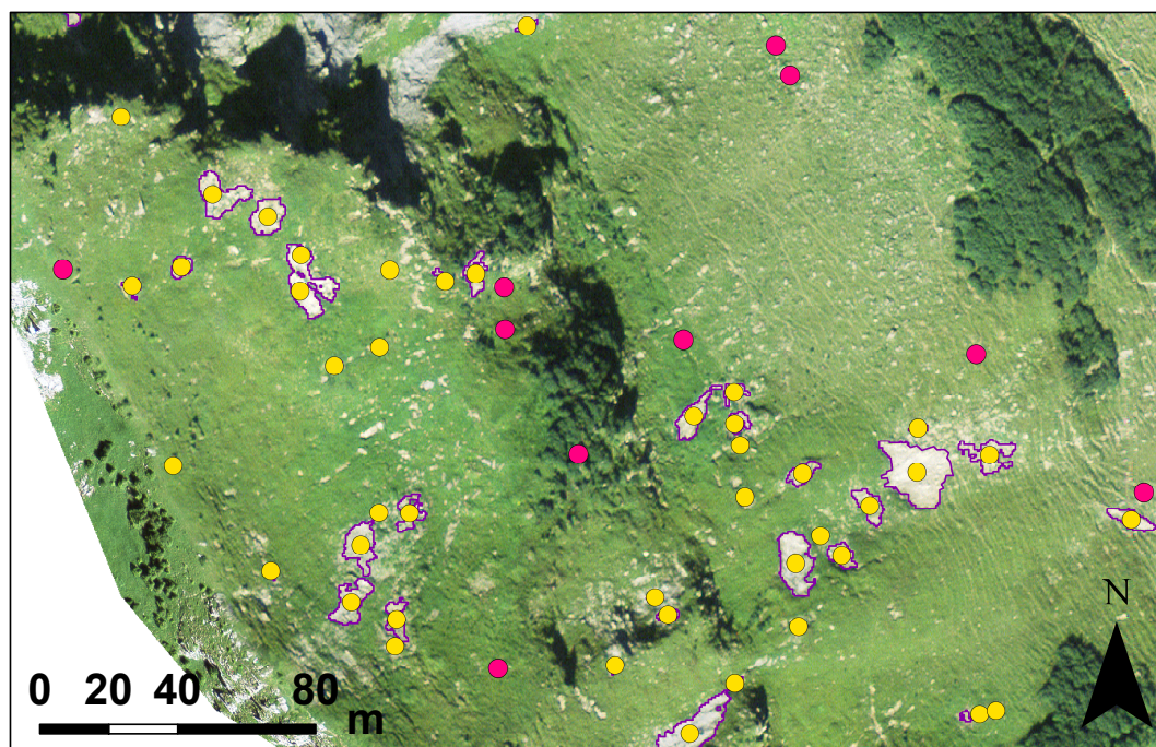
Figure 3. Example of mapped shallow landslides in the Turbach valley (purple). The centred points (yellow) represent shallow landslide locations for the Lasso model evaluation. Only sites with an area larger than 4 m 2 were used for the evaluation. Red points represent randomised non-landslide points. Aerial image (2013) obtained from Swisstopo.
