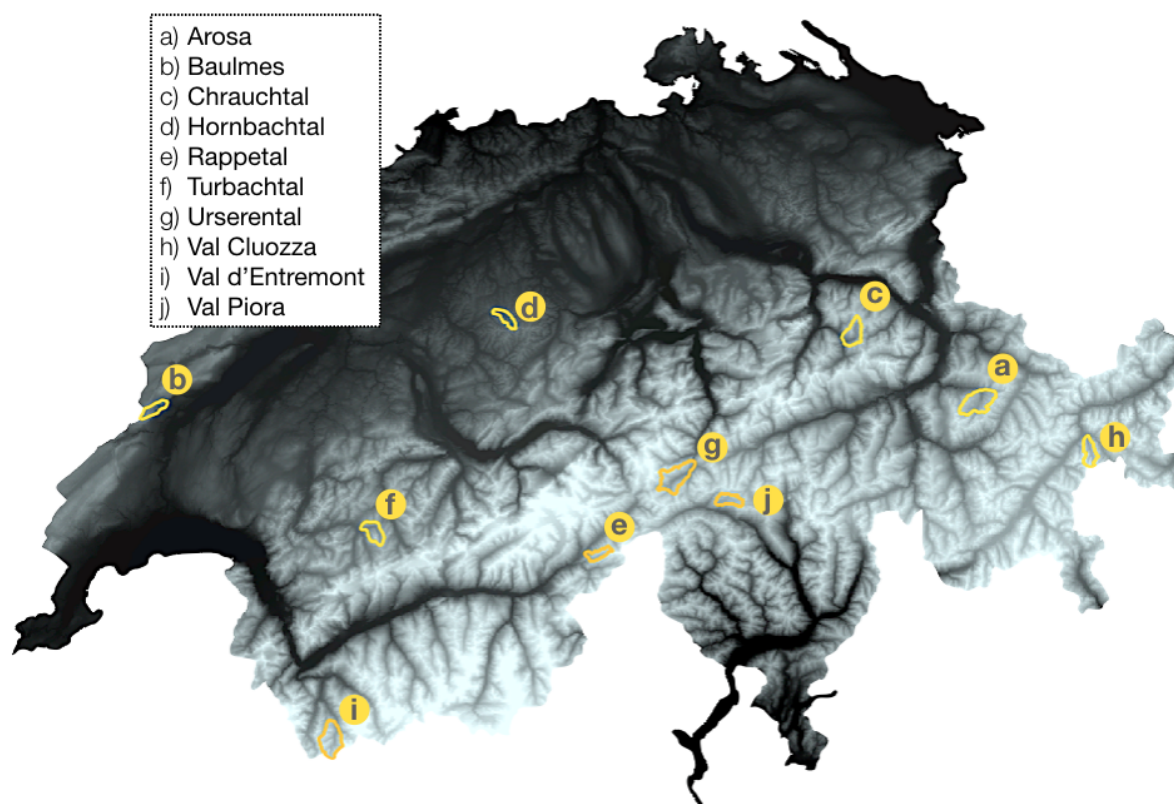
Figure 1. Map of Switzerland showing the 10 selected study sites (outlined in yellow). Colours of the map show lower elevations in dark and higher elevations in lighter colours.
