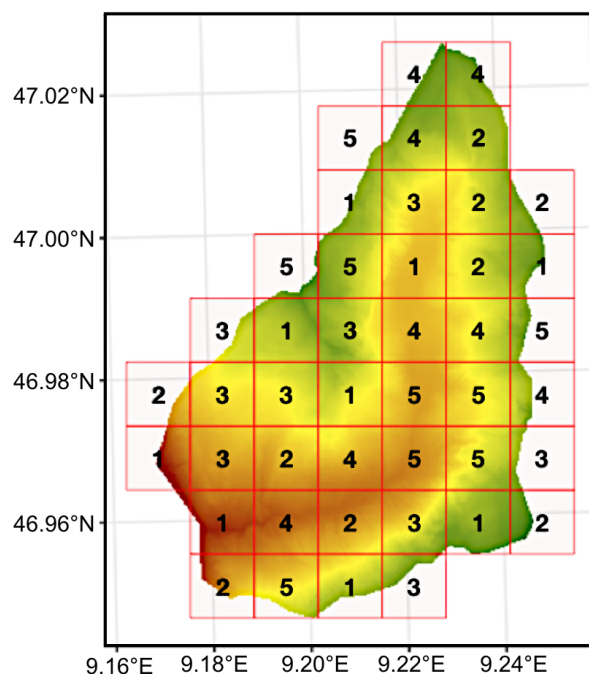
Figure 2. Spatial blocks for 5-fold cross-validation shown with the example of Chrauchtal. Blocks have a size of 1 km 2 . Blocks are assigned randomly and determined with the R-package blockCV (Valavi et al., 2019).
