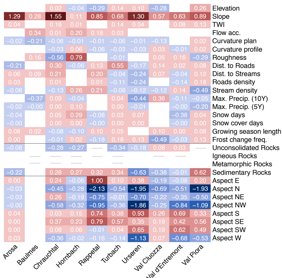
Figure 4. Heat-map displaying estimates of coefficients (median of 100 estimates) for all 10 sites. Note that not all geological rock classes are present at all sites (grey line). White boxes are equivalent to coefficients of zero and were therefore never selected for the models.
