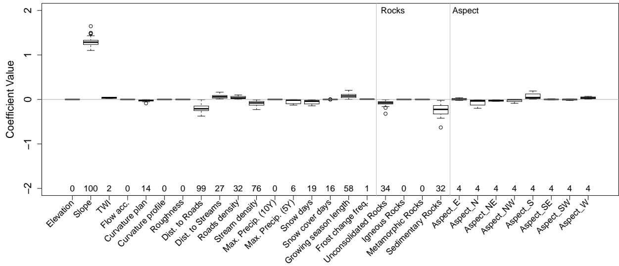
Figure S1: Coefficients Arosa
