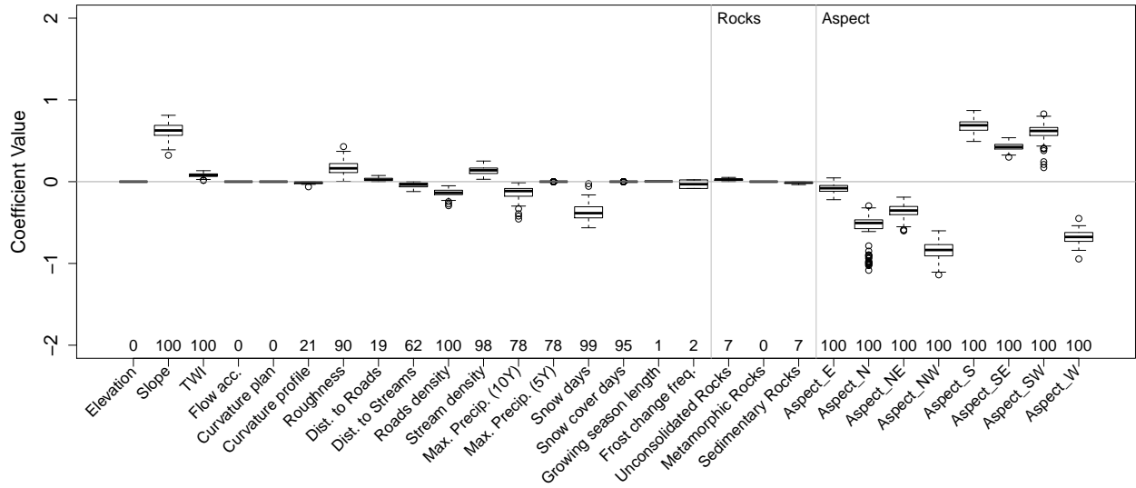
Figure S9: Coefficients Val d'Entremont
