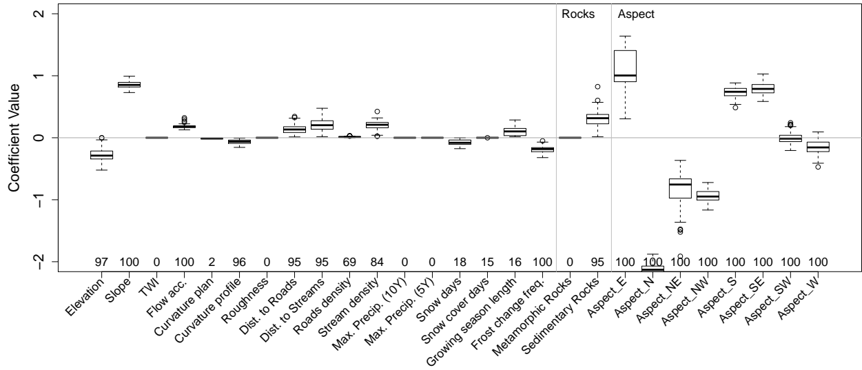
Figure S5: Coefficients Rappetal
