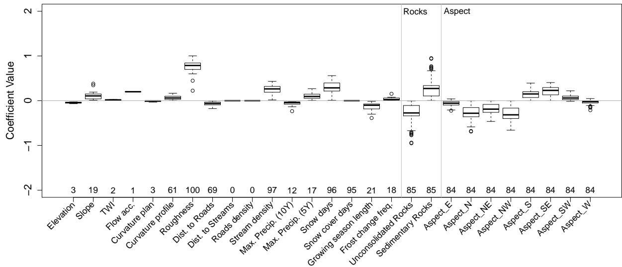
Figure S4: Coefficients Hornbachtal
