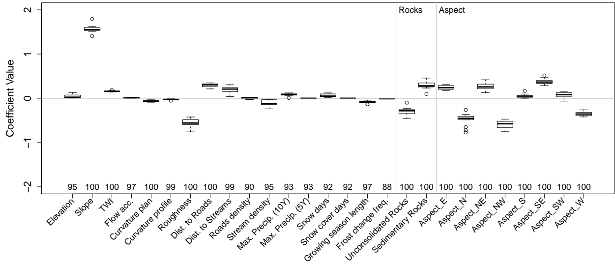
Figure S3: Coefficients Chrauchtal
