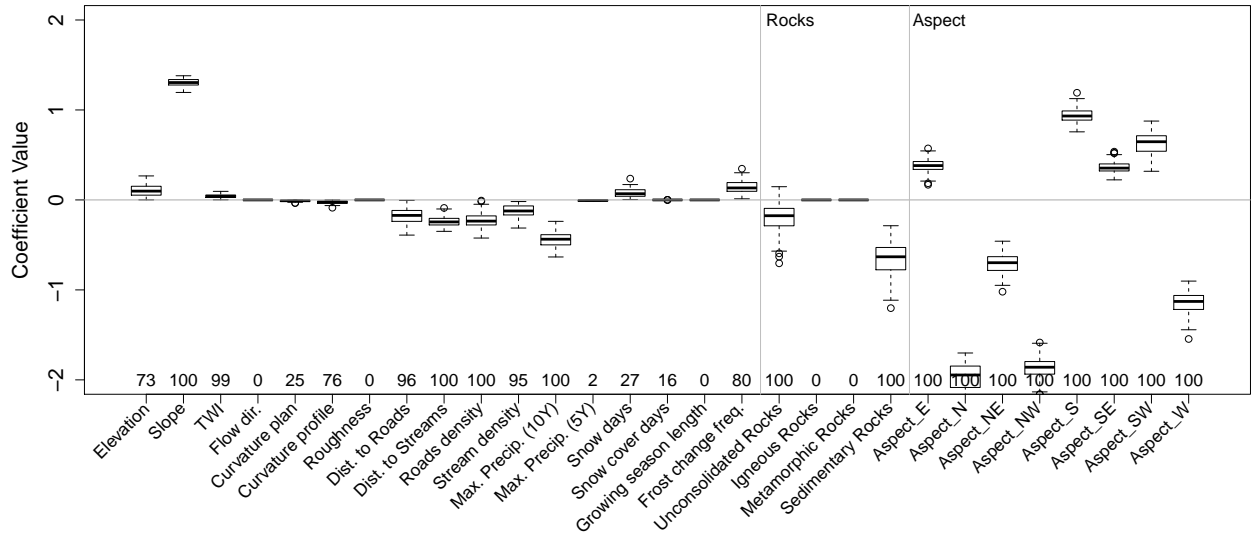
Figure S7: Coefficients Urserental
