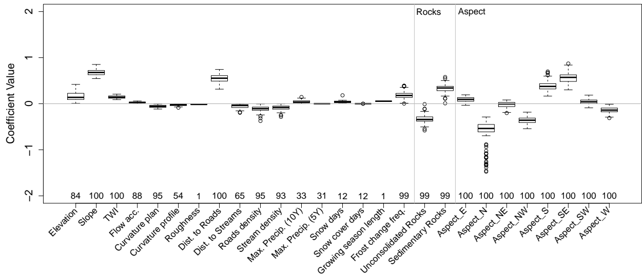
Figure S6: Coefficients Turbachtal
