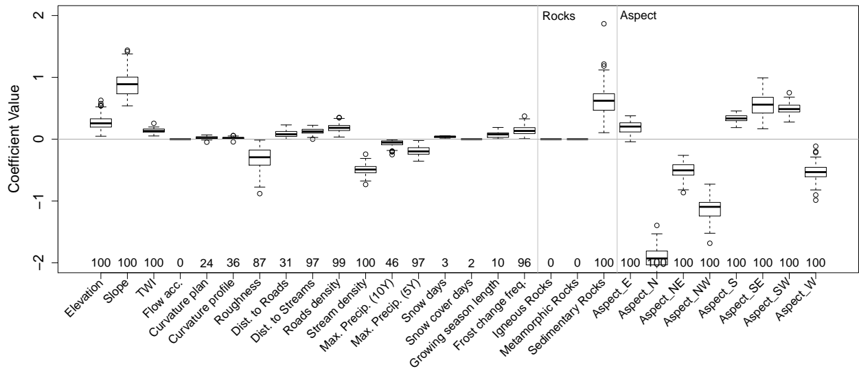
Figure S10: Coefficients Val Piara
