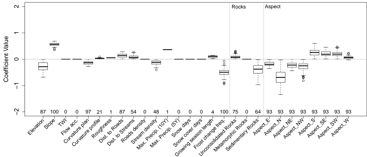
Figure S8: Coefficients Val Cluozza
