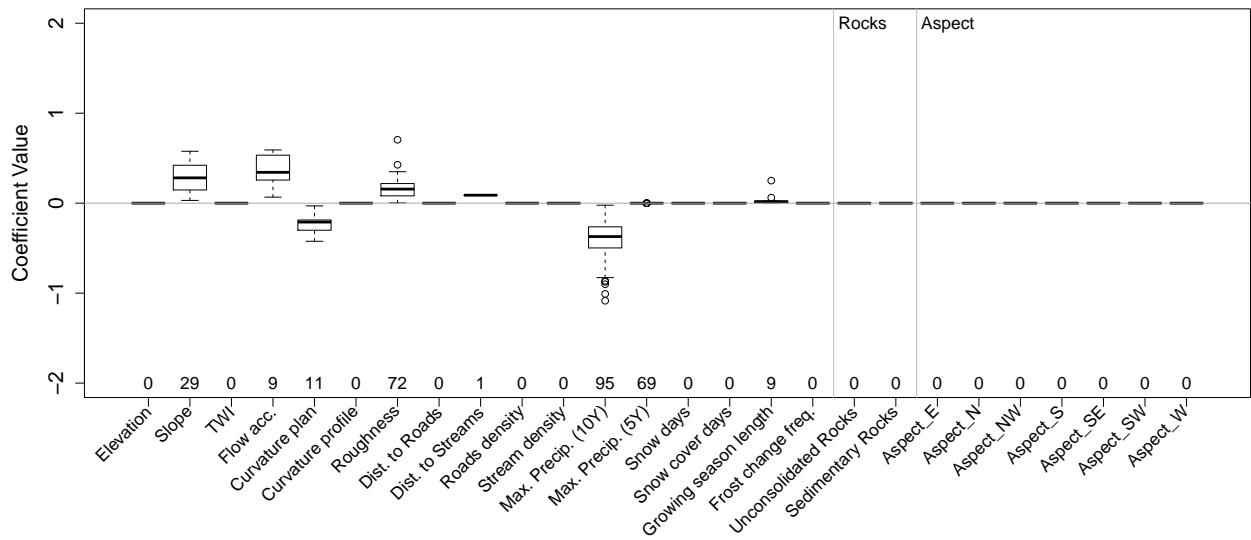
Figure S2: Coefficients Baulmes
