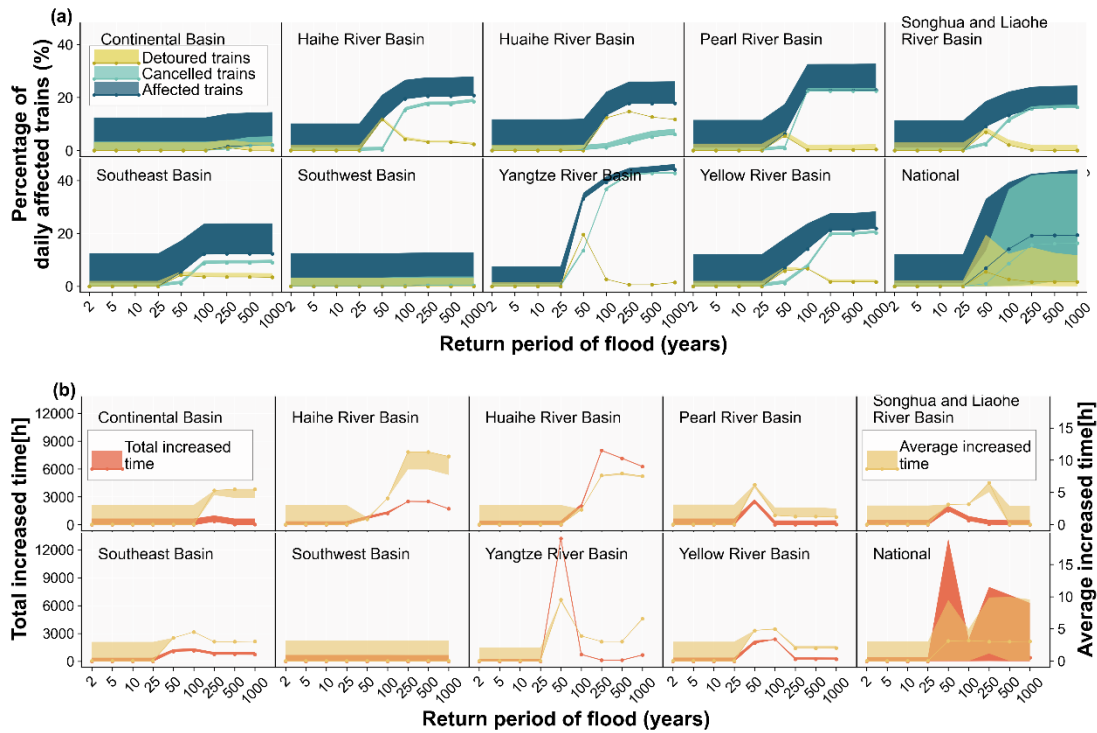
Fig. 7 System vulnerability curves induced by river floods from the national flood event set
