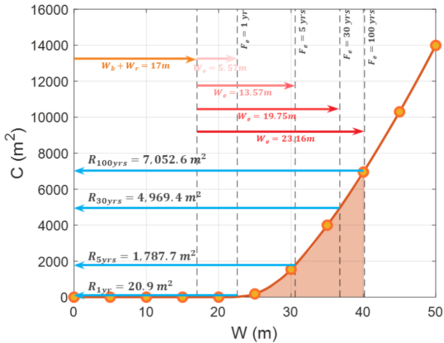
380 Figure 13: Estimation of combined potential erosion risk using the CPERC for Bongpo-Cheonjin Beach.
