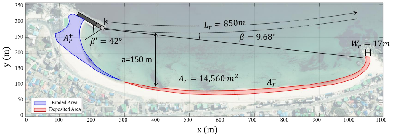
Figure 10: Calculation of PREA at Bongpo-Cheonjin Beach on image courtesy of National Geographic Information Institute (MOF, 2020).
