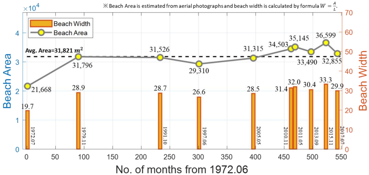
320 Figure 9: Variations of beach area and width for Bongpo-Cheonjin Beach using aerial photographs.
