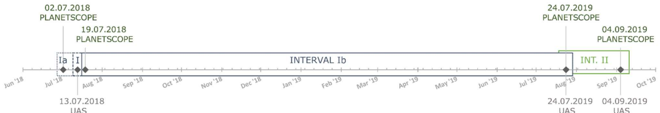
Figure 4 Acquisition dates of UAS and PlanetScope images within the investigated time period. Calculated interval I for UAS images (13.07.2018–24.07.2019, 376 d) and interval Ib for PlanetScope images (19.07.2018–24.07.2019, 370 d), interval II for UAS and PlanetScope images (24.07.2019–04.09.2019, 42 d). Note: Ia PlanetScope interval was discarded.
