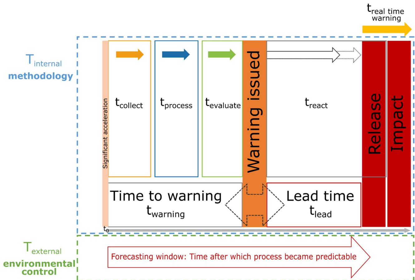
135 Figure 1 The novel conceptual approach for lead time, time to warning and the forecasting window for optical image analysis.
