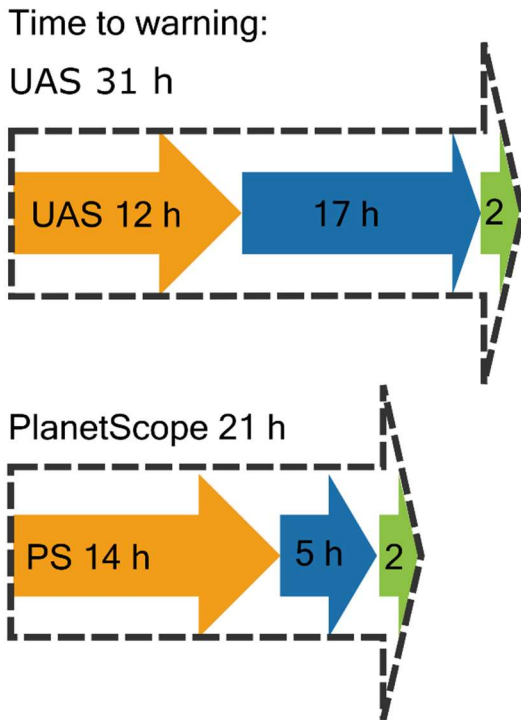
405 Figure 7 Time to warning is composed of three phases: time to collect, to process and to deliver. Time to warning (subsequent to acceleration) is 21 h for PlanetScope and 31 h for UAS. Thus, any hazard process that takes longer than 21/31 h to prepare the release and impact can be forecasted.
