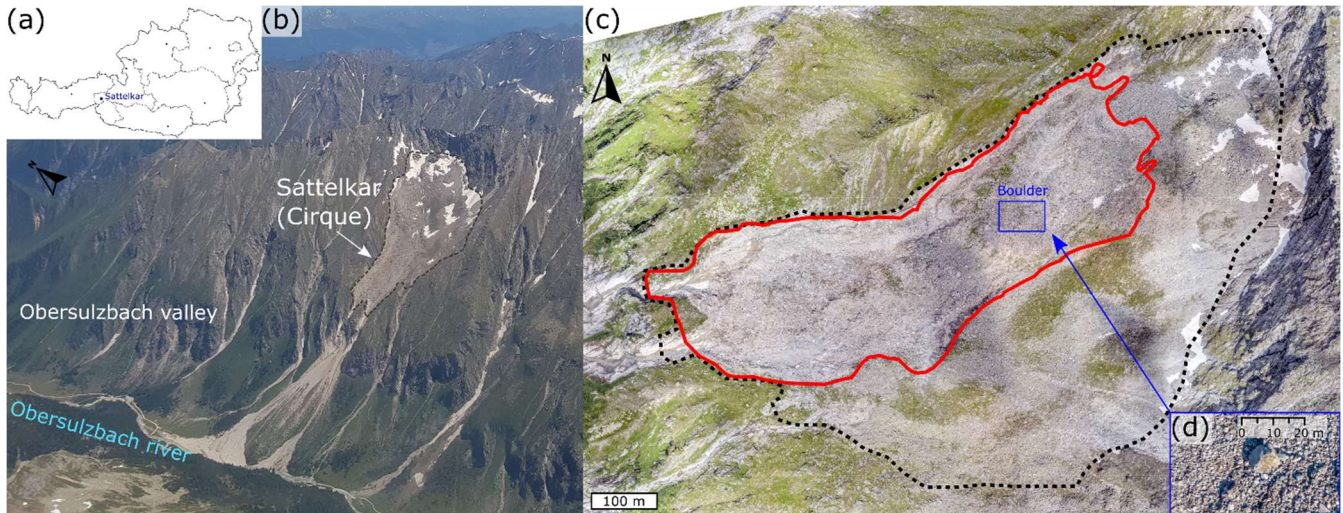
Figure 2 (a) Overview map Austria (Österreichischer Bundesverlag Schulbuch GmbH & Co. KG and Freytag-Berndt & Artaria KG, Wien). (b) Sattelkar, 30.6.2019 with the debris cone of the 2014 debris flow event and (c) UAS orthophoto (04.09.2019, 1:1.000) showing boulder sizes of 5–10 m used for manual motion tracking, (d) active boulder blocks from the central Aol.
