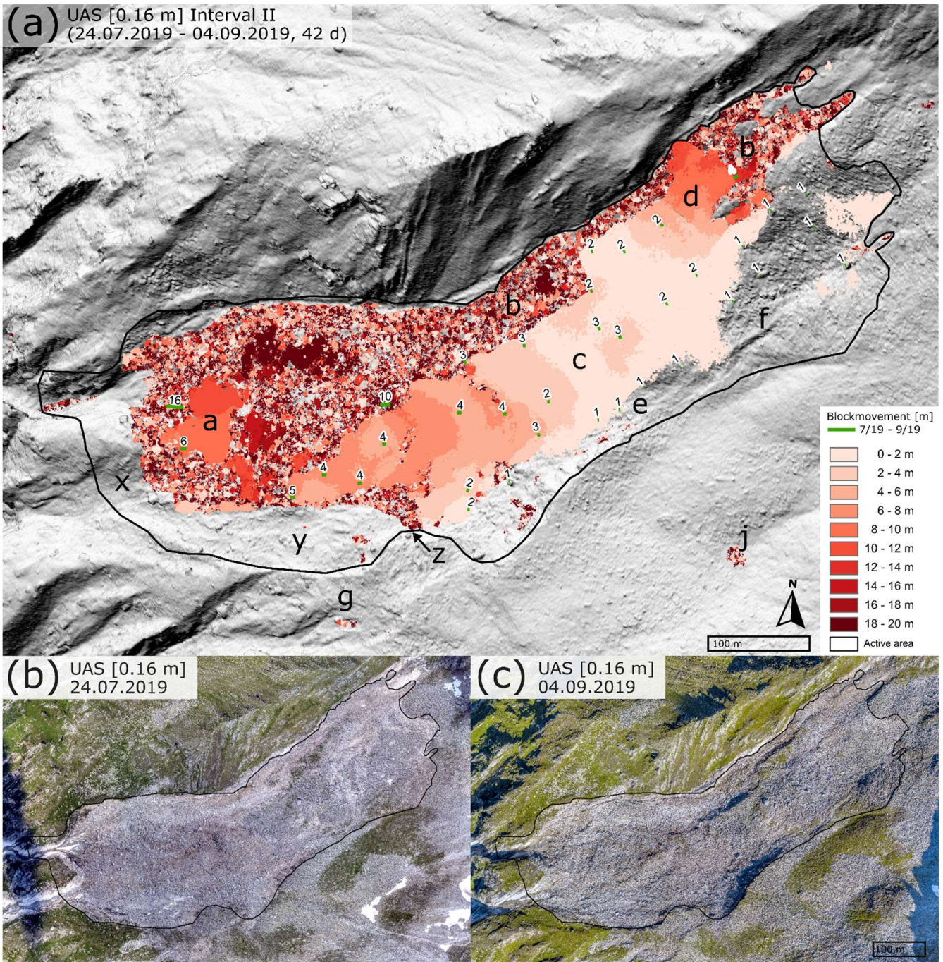
Figure 6 (a) Displacement derived from UAS data at 0.16 m resolution for interval II (24.07.2019–04.09.2019, 42 d) combined with boulder trajectories (in metres) manually measured in the UAS orthophotos in the same time period. The solid black line represents the boundary of the active landslide based on field mapping. Background: UAS hillshade, 24.07.2019 (0.08 m), orientation -3^\circ from north. UAS orthophotos at 0.16 m resolution for the master (b) and slave image (c) of the corresponding time interval.
