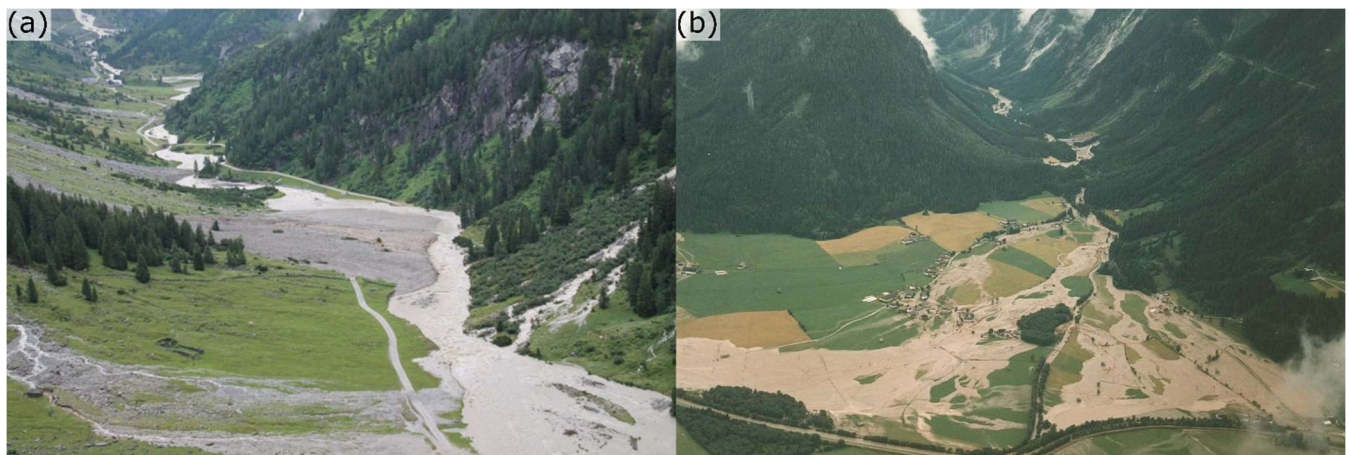
Figure 3 Obersulzbach valley, flood event September 2014. (a) Flooding situation in the Obersulzbach valley with the Sattelkar landslide cone deposit (image centre). (b) Flood area at the valley mouth in Sulzau and Schaffau. The Salzach river is at the bottom of the image. ©Salzburger Nachrichten/Anton Kaindl.
