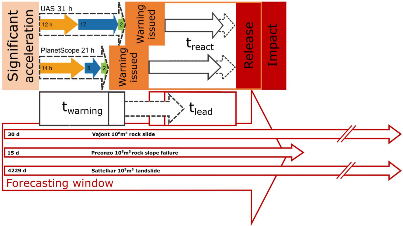
Figure 8 Conceptual approach with estimated t_{\text{warning}} for UAS and PlanetScope. Phases of collection, processing and evaluation (indicated as arrows of relative length in orange, blue and green, respectively) (see phases in Fig. 1 and Fig. 7) with their total duration time (grey dashed arrows). In t_{\text{warning}} , one additional observation requires in sum 31 h for UAS and 21 h for PlanetScope data. Above, major landslides are compared from the onset or displacement detection (solid line) (Petley and Petley, 2006; Anker et al., 2016; Sättele et al., 2016).
