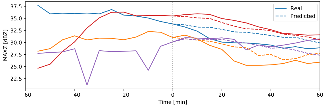
Figure 3. Examples of the prediction of MAXZ. The figure shows the curves of observed and predicted MAXZ (the mean over the 25-km diameter region of interest) for four different tracked centers. The solid lines show the development of MAXZ while the dashed lines show the predictions after t = 0 .
