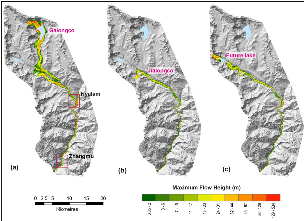
Figure 3: Modelled GLOF flow heights for worst-case scenarios from (a) Galongco, (b) Jialongco (JC-L), and (c) the potential future lake. The location of Nyalam and Zhangmu towns are indicated by the red boxes in (a).
