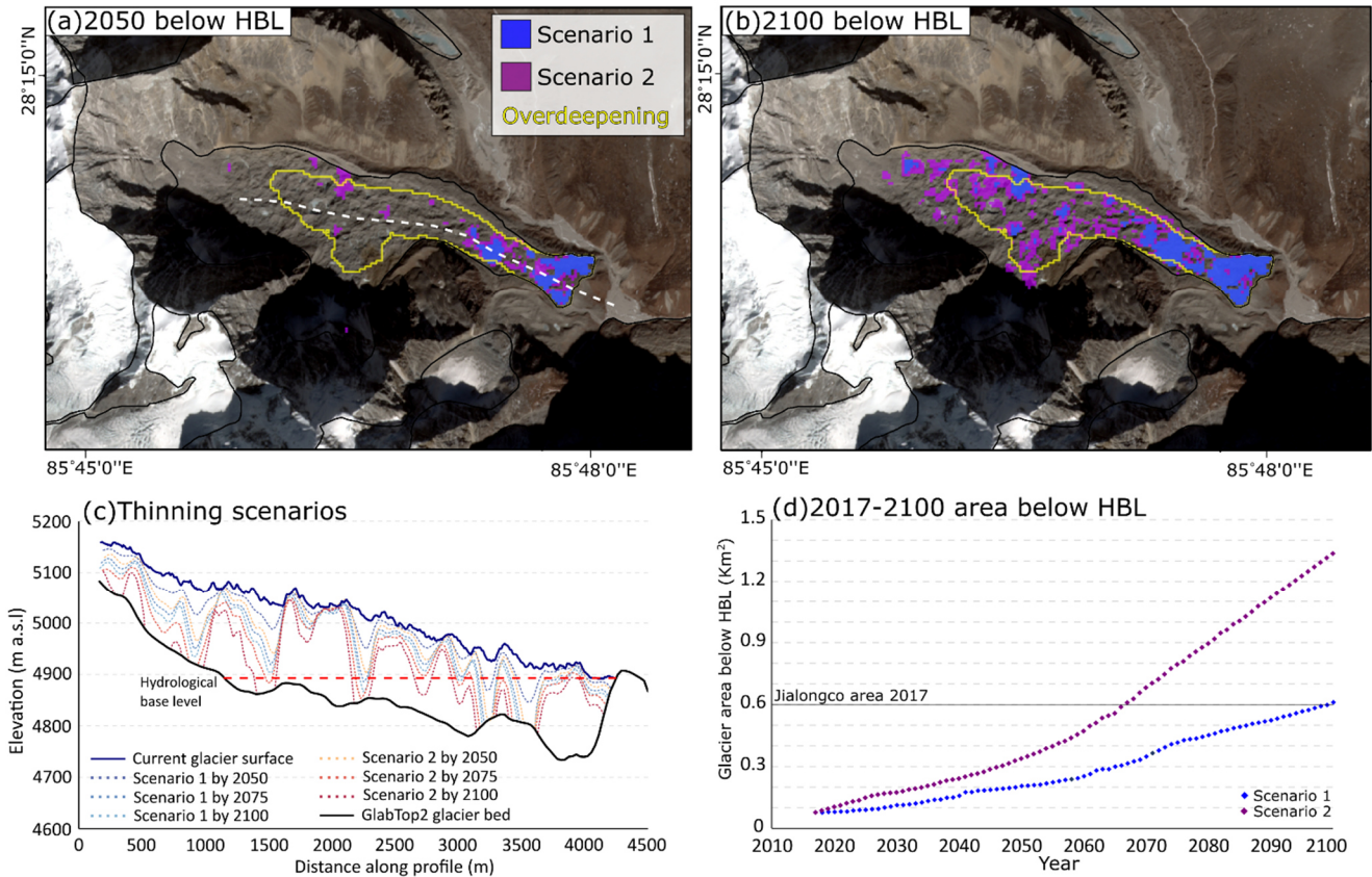
475 Figure 8: Meltwater ponding (if elevation < the hydrological base level of the glacier) by 2050 (a) and 2100 (b) under different scenarios of thinning for glacier RGI60-15.09475. Background imagery is modified Copernicus Sentinel data (14-10-2021), processed by the European Space Agency. Glacier surface elevation profiles taken along the dashed profile on panel (a) under each scenario of thinning are also shown in panel (c). The full timeline of supraglacial lake area expansion is shown in (d). The area within the yellow polygon shows the location of a bed overdeepening (1.54 km 2 ) predicted by GlabTop. Ice flow is from left to right in a-c.
