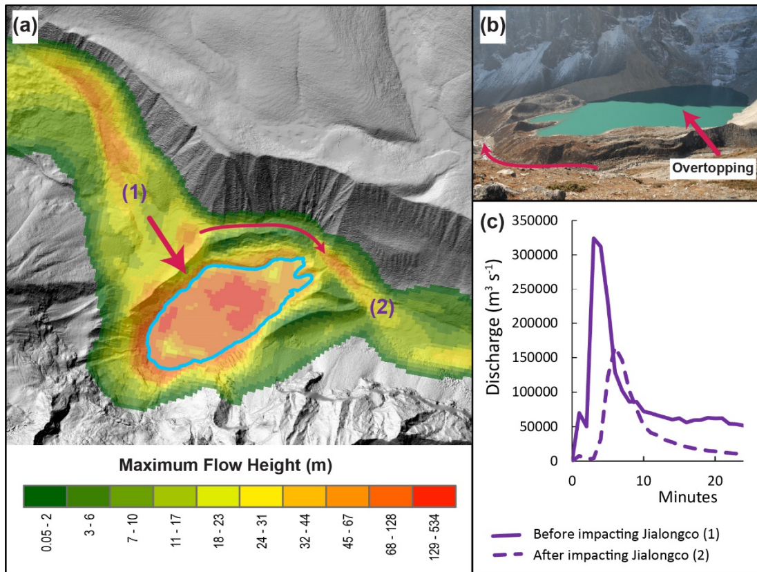
Figure 5: (a) Modelled GLOF flow heights for an outburst event from the potential new lake, showing area of pooling and overtopping into Jialongco. Background DEM generated based on Pleiades data 15 Oct 2018 © CNES and Airbus DS. The moraine height at the point where overtopping is illustrated in the photo (b) is around 40 m (Photo: O. King, October 2018). (c) Flow hydrographs immediately upstream (1) and downstream (2) of Jialongco are simulated with r.avafLOW. Note that the simulation is based on the post-lowering lake bathymetry and dam geometry of Jialongco (JC-L).
