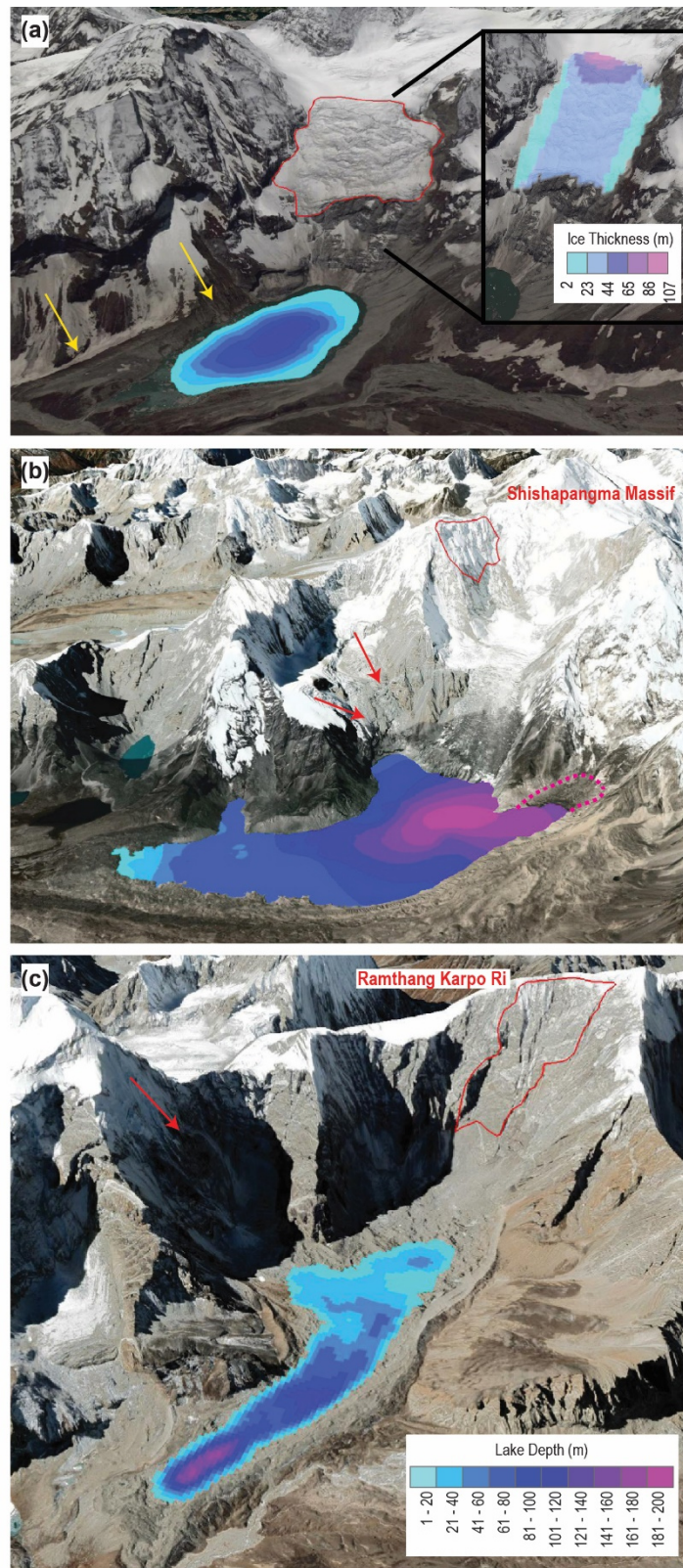
340 Figure 2: Rock/ice avalanche starting zones (in red) used as input scenarios for the modelling of outburst flood process chains from the 3 lakes (see Table 1 for details). (a) Jialongco: The inset shows the GlabTop modelled ice thickness of the ice avalanche source area, and yellow lines indicate the steep lateral moraine walls also threatening the lake (see also Fig. 9). (b) Galongco: Large rock/ice avalanche source area outlined in red, while arrows indicate smaller sources areas of unstable ice, with possible future expansion of the lake shown by the dashed line. (c) Projected future lake: Large rock avalanche source area outlined in red, while arrow indicates
