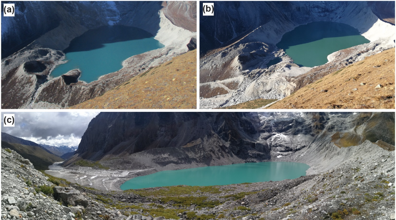
560 Figure 9: Images taken of Jialongco in (a) October 2018 showing the natural state of the lake, (b) October 2020 and (c) September 565 2021, showing the engineering work that has been undertaken in the outlet area, lowering the lake level, removing much of the frontal moraine, and establishing a stable, armoured outlet channel. Photos: T. Bolch (a) and G. Zhang (b, c).
