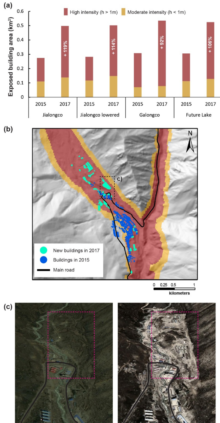
440 Figure 6: (a) Built area in Nyalam exposed to modelled GLOF intensity levels for the three assessed lakes, showing the effect of rapid infrastructural development between 2015 and 2017. The percentage indicates the increase in built area within the high intensity zone. (b) Modelled intensities for the Galongco outburst scenario showing the recent expansion of infrastructure, as mapped from © Google Earth imagery from June 2015 (c - left) and October 2017 (c - right). A notable area of infrastructure development just upstream of the main bridge is highlighted in the dashed rectangle.
