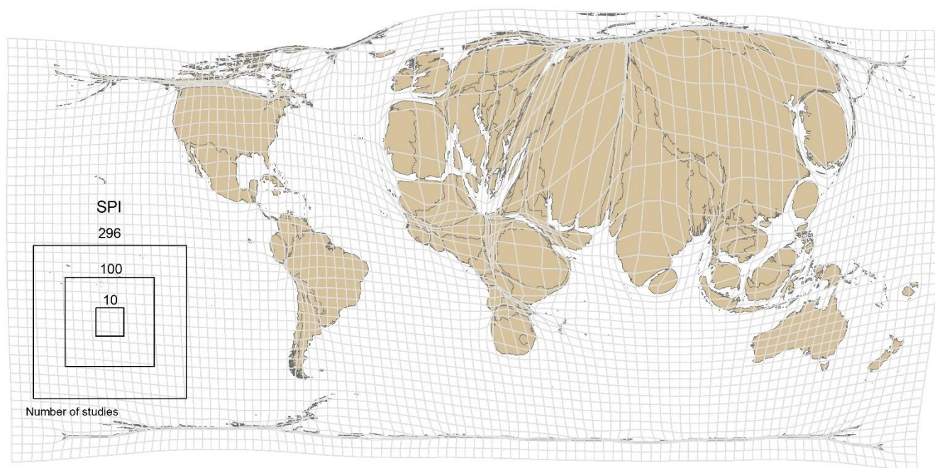
285 Figure 6: Contiguous cartograms (Gastner-Newman) of the world with each country rescaled in proportion to the number of studies on Scopus related to drought and the SPI
