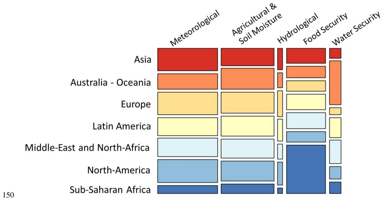
Figure 04: Mosaic plot showing how frequently keywords, being the types of drought and impacts, were mentioned in the titles, abstracts, and keywords in drought-related studies on Scopus. The height (vertical) of each box indicates how frequently the keyword is used for each region (the frequency was scaled by the number of papers for each region, that is, the plots show the keyword frequency if all the regions had an equal number of papers). The width (horizontal) of each box indicates the relative frequency of each keyword.
