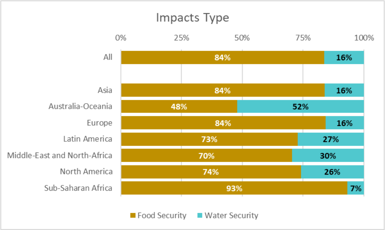
145 Figure 03: Barplot showing the proportion of food and water security studies related to drought per region of the world on Scopus.
