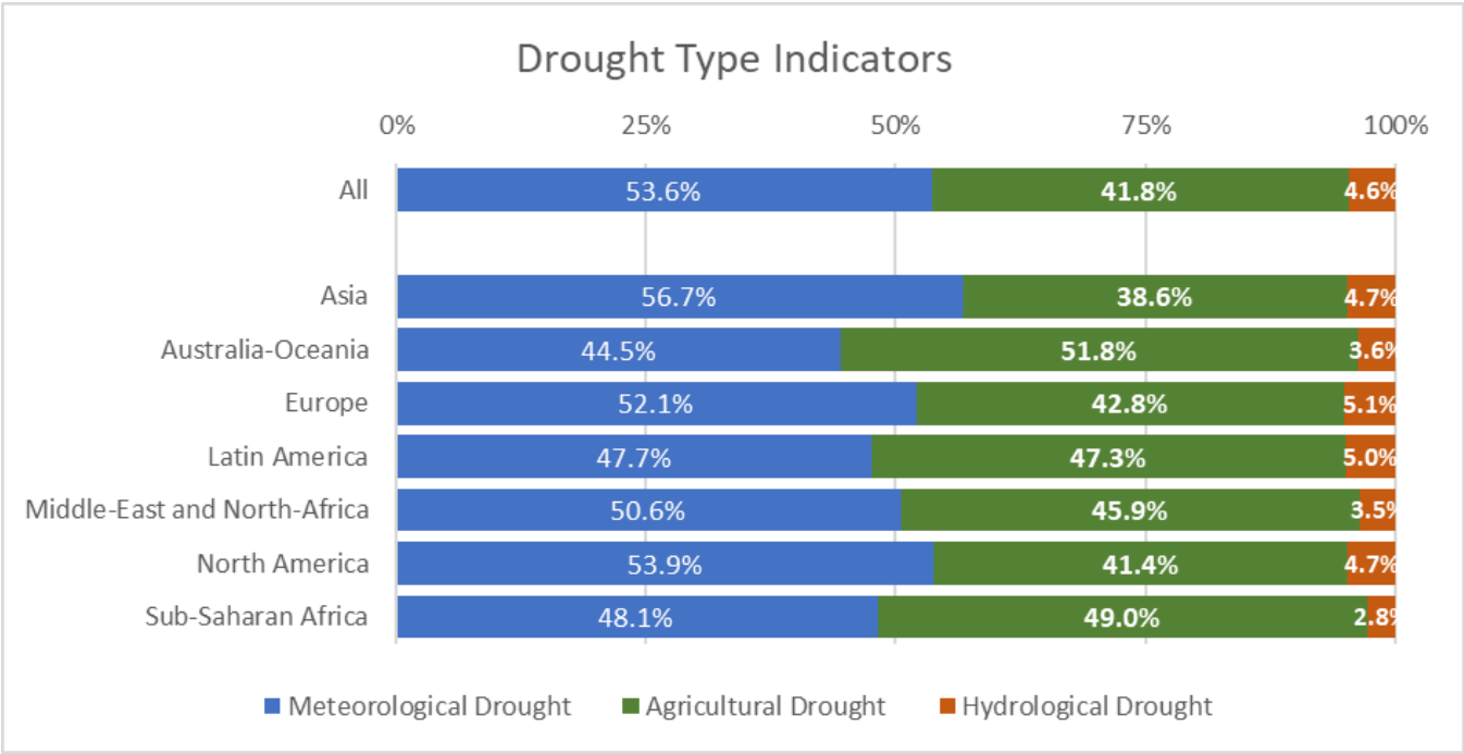
125 Figure 02: Barplot showing the proportion of drought type studies per region of the world, according to the drought indices referred to in the title, abstract and keywords of drought-related studies on Scopus.
