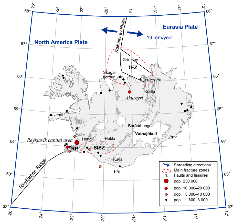
Figure 1. The ICCEL region, 62°–68°N and 12°–26°W. The figure shows place names in Iceland mentioned in the article. Towns and villages with 2020 population of at least 800 are also indicated as well as the Tjörnes Fracture Zone (TFZ), the South Iceland Seismic Zone (SISZ), and the Reykjanes Peninsula (RP)
