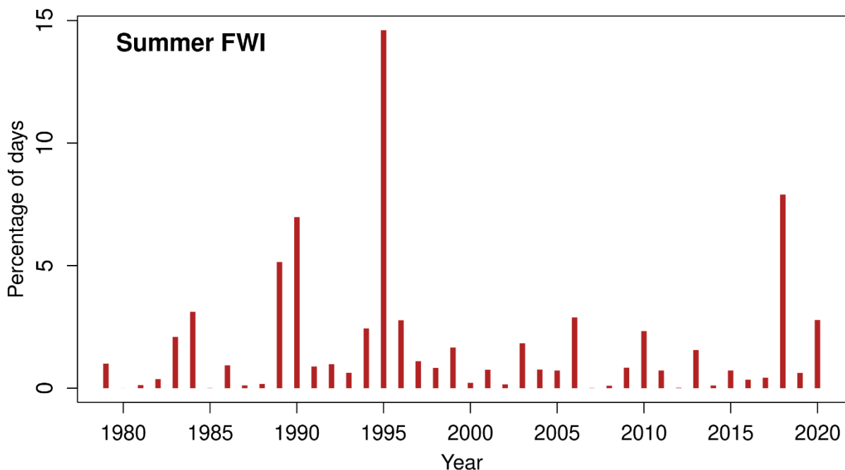
305 Figure 5: Annual percentage of summer (June-July-August) days, 1979–2020, averaged over the UK, with ‘very high’ fire danger (FWI > 17.35), based on ERA5 reanalysis data.
