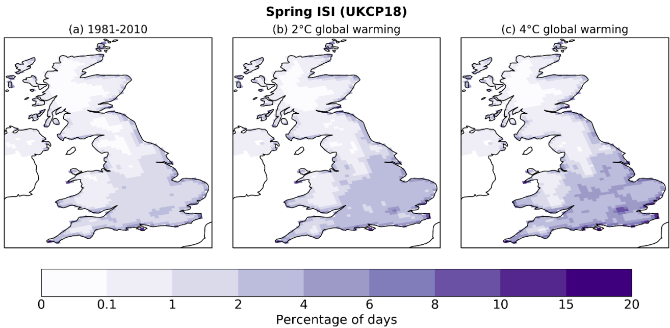
Figure 9: Percentage of spring days with ‘high’ fire danger (ISI > 5) over the UK, based on the UKCP18 12 km data averaged over the 12 ensemble members. a) Historical period (1981–2010), b) 2°C global warming, c) 4°C global warming. The colour bar is the same as in Fig. 8a.
