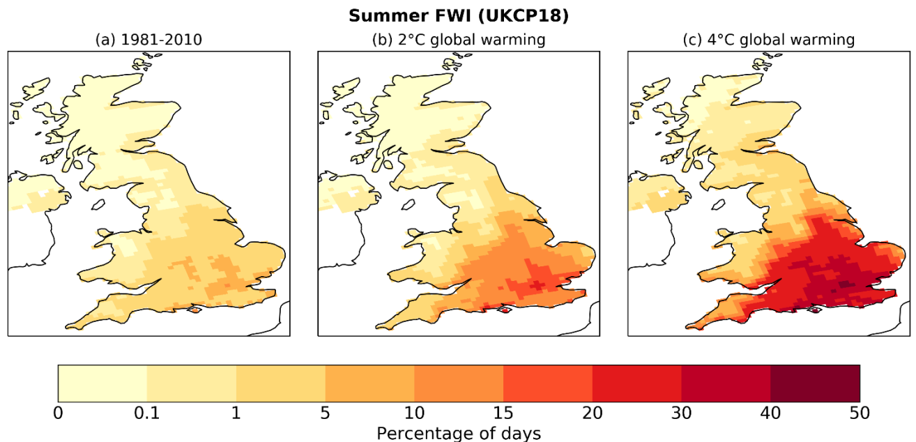
Figure 10: Percentage of summer days with ‘very high’ fire danger (FWI > 17.35) over the UK, based on the UKCP18 12 km data averaged over the 12 ensemble members. a) Historical period (1981–2010), b) 2°C global warming, c) 4°C global warming. The colour bar is the same as in Fig. 8b.
