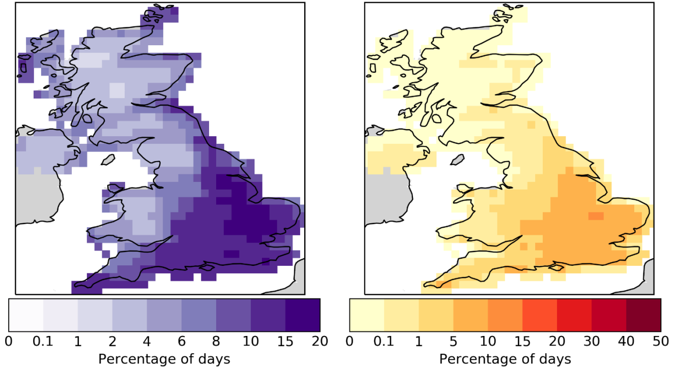
Figure 8: Percentage of days with dangerous fire weather for a) spring (ISI > 5; at least ‘high’); b) summer (FWI > 17.35; at least ‘very high’). Based on the ERA5 reanalysis data for the 1981–2010 period.
