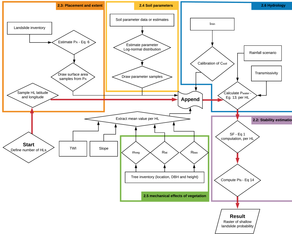
Figure 1. Flowchart of the computational steps in SlideforMAP. Separate sections are outlined in colors. The central workflow is highlighted.
