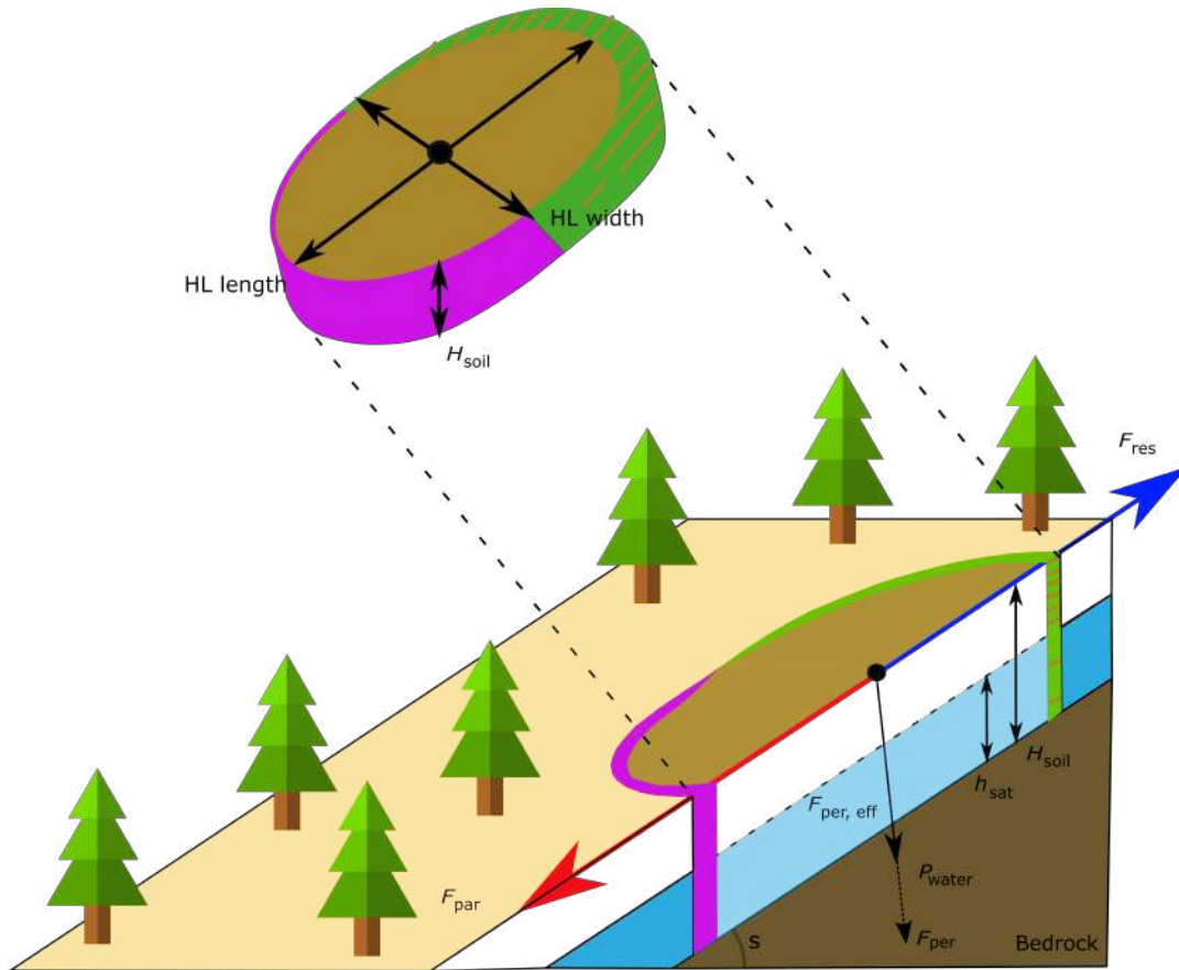
Figure 2. Schematic overview of the forces acting upon a hypothetical landslide, as assumed in SlideforMAP. The blue arrow, F_{res} , indicates the stabilizing forces and the red arrow, F_{par} , indicates the destabilizing forces. Lateral root reinforcement only acts upon the green part of the hypothetical landslide, where tension takes place. In purple is the compression zone in the shallow landslide. Basal root reinforcement and soil shear strength act on the whole potential failure surface.
