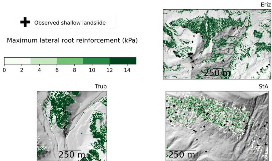
Figure 9. The spatial distribution of maximum root reinforcement (equation 8) in the study areas as used in SlideforMAP. Source of hillshade: Federal Office of Topography Swisstopo (Swisstopo, 2018)
