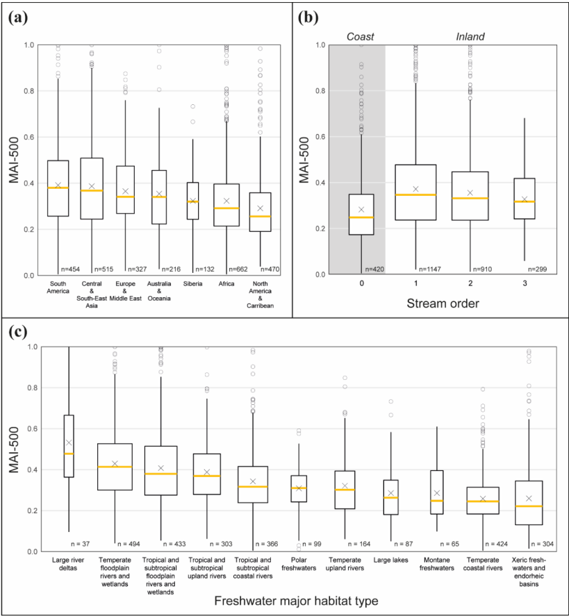
370 Figure 4: How the model agreement between GFPLAIN, GAR-500 and JRC-500 varies with (a) geographic region, (b) river stream order, and (c) freshwater major habitat type. The model agreement index ranges between 0 % (no agreement) and 100 % (full agreement) and was here calculated for all the river basins of the world that are covered by all three models. The box hinges correspond to the first and third quartile and the yellow line correspond to the second quartile (median value). The mean value is indicated with a cross. The whiskers extend from the box hinges with maximum lengths equal to the inter-quartile range multiplied with a factor of 1.5. Values outside of the whiskers are indicated with dots. The number of river basins corresponding to each group
