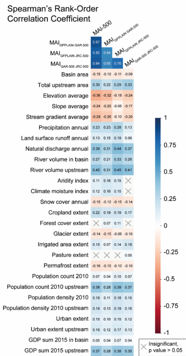
450 Figure 5 Spearman rank-order correlation coefficients between the flood model agreement scores and 27 hydro-environmental attributes. Wetter conditions due to climate (precipitation, land surface runoff) and river size (e.g. river volume, natural discharge) are positively associated with the model agreement between the flood maps. Topographic variables like high altitude (elevation) and steep slope (e.g. slope and stream gradient) are negatively associated with the model agreement, especially between GFPLAIN and GAR-500. The correlogram is using a hierarchical clustering order. Please note that the Aridity index increases with humidity.
