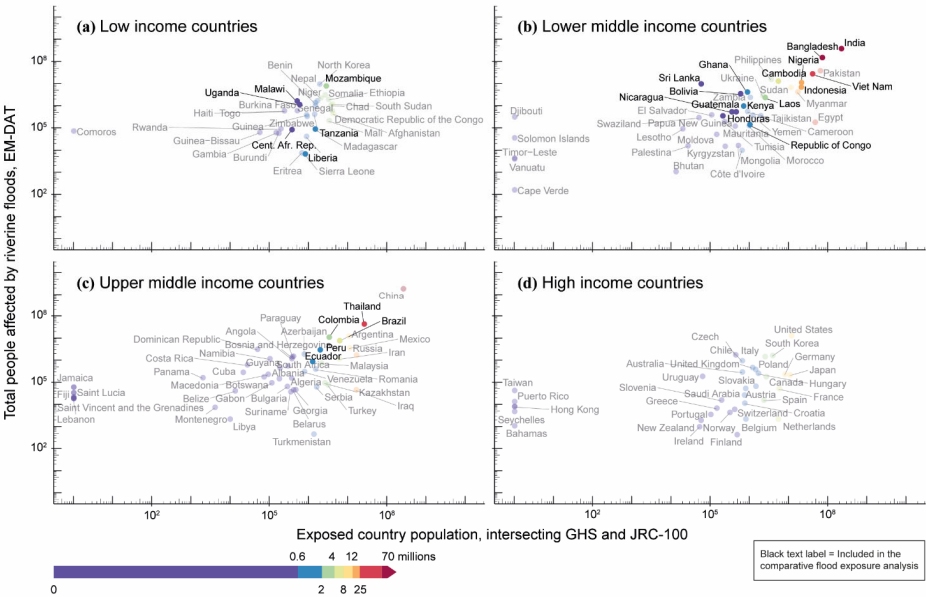
Figure 1: Flood risk-exposure in the 26 countries for which we conducted the comparative riverine flood exposure analysis, here marked with black text labels. Flood risk is here represented as the combination of the country population within the 100-year flood hazard map (intersecting the Global Human Settlement Population count for 2015 with the JRC flood hazard map) and actual disaster reports of people affected by riverine floods 1900-2020 as included in the Emergency Events Database EM-DAT. Please note that the axes have logarithmic scales. The country income classification is based on GNI per capita for the year 2015, given by the World Bank.
