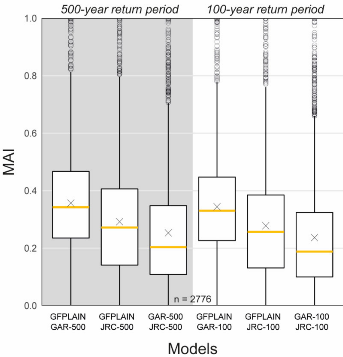
310 Figure 2 Pairwise evaluation of model agreement between the hydrogeomorphic floodplain map GFPLAIN and the flood hazard 315 maps GAR and JRC, with 100- and 500-year return period. The box hinges correspond to the first and third quartile and the yellow line correspond to the second quartile (median value). The mean value is indicated with a cross. The whiskers extend from the box hinges with maximum lengths equal to the inter-quartile range multiplied with a factor of 1.5. Values outside of the whiskers are indicated with dots. A higher return period shows higher agreement with GFPLAIN, but the choice of flood model influences the level of agreement even more. The flood hazard maps GAR and JRC show the lowest level of agreement. The index has here been calculated for the 2776 river basins across the world that are covered by all three models.
