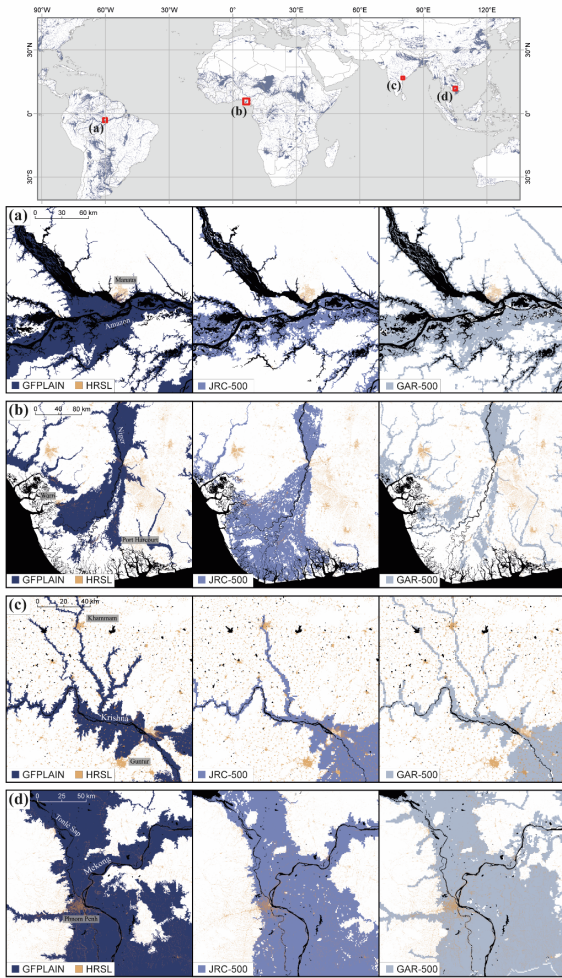
Figure 8 Spatial patterns of the hydrogeomorphic floodplain map GFPLAIN compared to the flood hazard maps JRC and GAR with a 500-year return period, for the rivers (a) Amazon in Brazil, (b) Niger in Nigeria, (c) Krishna in India, and (d) the Mekong in Cambodia. The brown pixels indicate settlements mapped with the High Resolution Settlement Layer. The black pixels indicate the permanent water mask. GFPLAIN and GAR cover more rivers compared to JRC due to having lower thresholds of upstream drainage area. There is a major discrepancy between the treatment of coastal regions between the individual models, here particularly evident for the Niger Delta (b).
