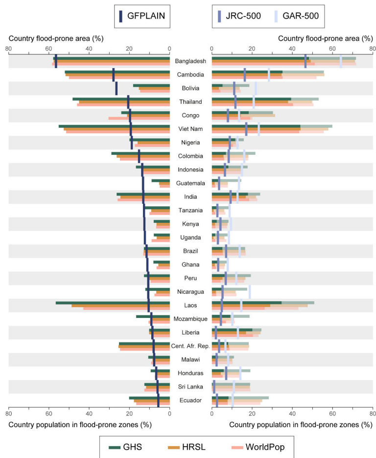
Figure 7 Riverine flood exposure estimates, aggregated at country level, using the hydrogeomorphic floodplain map GFPLAIN (bars on the left) and the flood hazard maps of JRC (bars on the right) and GAR (shaded bars on the right) with a 500-year return period. The green, orange and pink horizontal bars indicate the percentage country population in flood-prone zones using the population maps Global Human Settlement, High Resolution Settlement Layer and WorldPop respectively. The vertical blue bars indicate the percentage of land area that is flood-prone. Country boundaries are outlined by the GAUL 2015 dataset and permanent water is masked by the product MOD44W.
