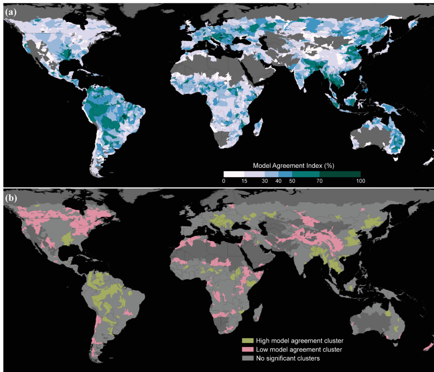
Figure 3: (a) Spatial distribution of MAI-500, the model agreement between the hydrogeomorphic floodplain map GFPLAIN and the flood hazard maps GAR and JRC with a 500-year return period. The model agreement index ranges between 0 % (no agreement) and 100 % (full agreement) and was here calculated for all the river basins of the world that are covered by all three models. (b) Local clusters of river basins with high or low agreement values relative to the mean, identified from the spatial autocorrelation analysis.
