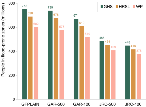
Figure 6 Total exposed population (millions) across all 26 countries, comparing the hydrogeomorphic floodplain map GFPLAIN with the flood hazard maps GAR and JRC with 100- and 500-year return periods. The population estimates are given by the Global Human Settlement Layer, the High Resolution Settlement Layer and WorldPop. The floodplain map GFPLAIN yields the highest exposure estimates, even though GAR-500 covers a slightly larger total area. The choice of flood and population maps affect the results more than the choice of the return period.
