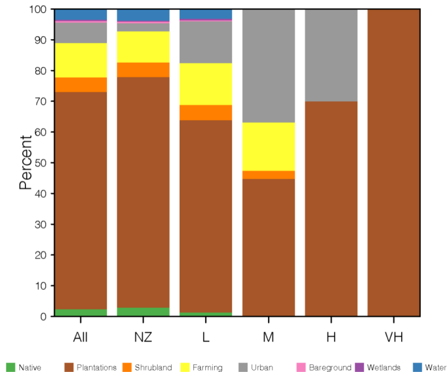
Figure 3 Land use (%) classified for the CMA according to the wildfire categories: Near Zero (NZ), Low (L), Moderate (M), High (H), Very High (VH) and All. “All”, represents the distribution of the land cover along the whole study area.
