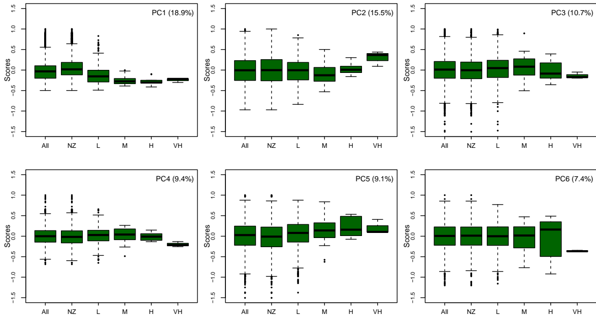
Figure 5. Boxplots showing the distribution of PC's weights according to the recurrence categories. "All" represents the distribution of each PC along the whole study area.
