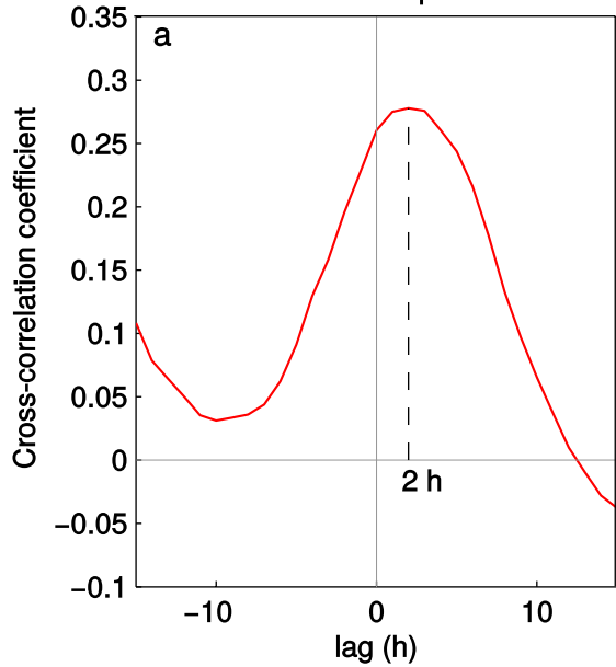
Rockfall / Air temperature
