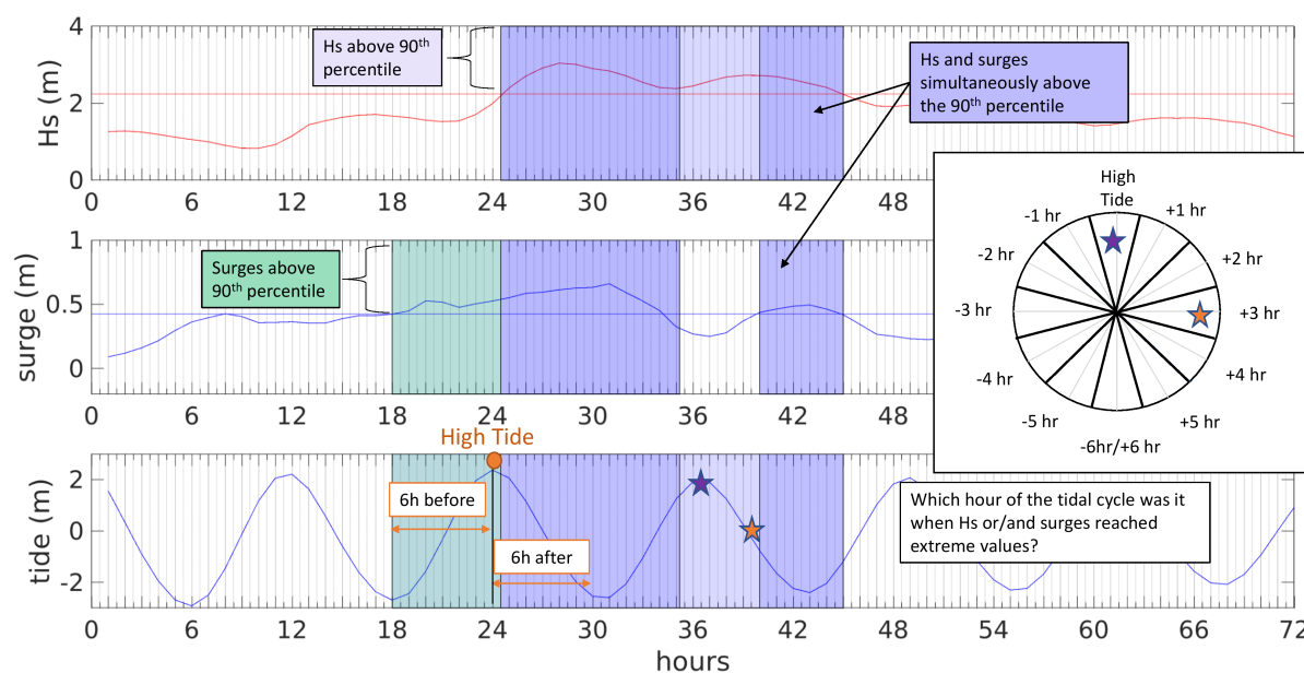
Figure 2. schematic example explaining the methodology used to evaluate the amount of extreme Hs and surges with respect to the tidal cycle. This example shows three day of the time series at one coastal point. The Hs values higher than the 90 th percentile (calculated over 3 months of data at the same point) are considered high. The closest tidal peak to each value is found. We then evaluate when each value occurred in the tidal cycle, from 6h before to 6h after high tide. The same is done for surges, and for cases in which Hs and surges are simultaneously higher than the respective 90 th percentile. The two stars indicate examples, where the extreme Hs occurred at high tide, and three hours after high tide.
