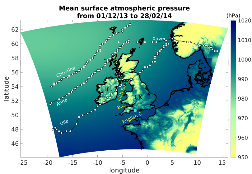
Figure 1. The UKC4 model domain with shading giving the UKC4 simulated mean surface atmospheric pressure during the 3 months of winter 2013/4. The figure also shows the estimated track of four storms during winter 2013 (storms Xaver 5/12/2013, Anne 3/01/2014, Christina 7/01/2014, and Ulla 14/02/2014). Tracks are obtained from the mean sea level pressure (MSLP) of hourly ERA5 reanalysis data. The white markers show the location of hourly minimum MSLP during the storm period. The red and blue dots show the locations of Solway Firth and Weymouth respectively, which are mentioned in the discussion.
