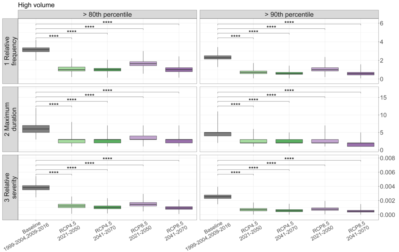
435 Figure 9 - Boxplots of relative frequency, maximum duration and relative severity metrics calculated from volume values greater than the 80 th and 90 th percentiles. The simulated volume values used for the metrics calculation resulted from the Monte Carlo approach by randomly sampling from the volume prediction bands. Symbol '****' refers to p-value \leq 0.0001 . For interpretation of the references to colour in this figure legend, the reader is referred to the web version of this article.
