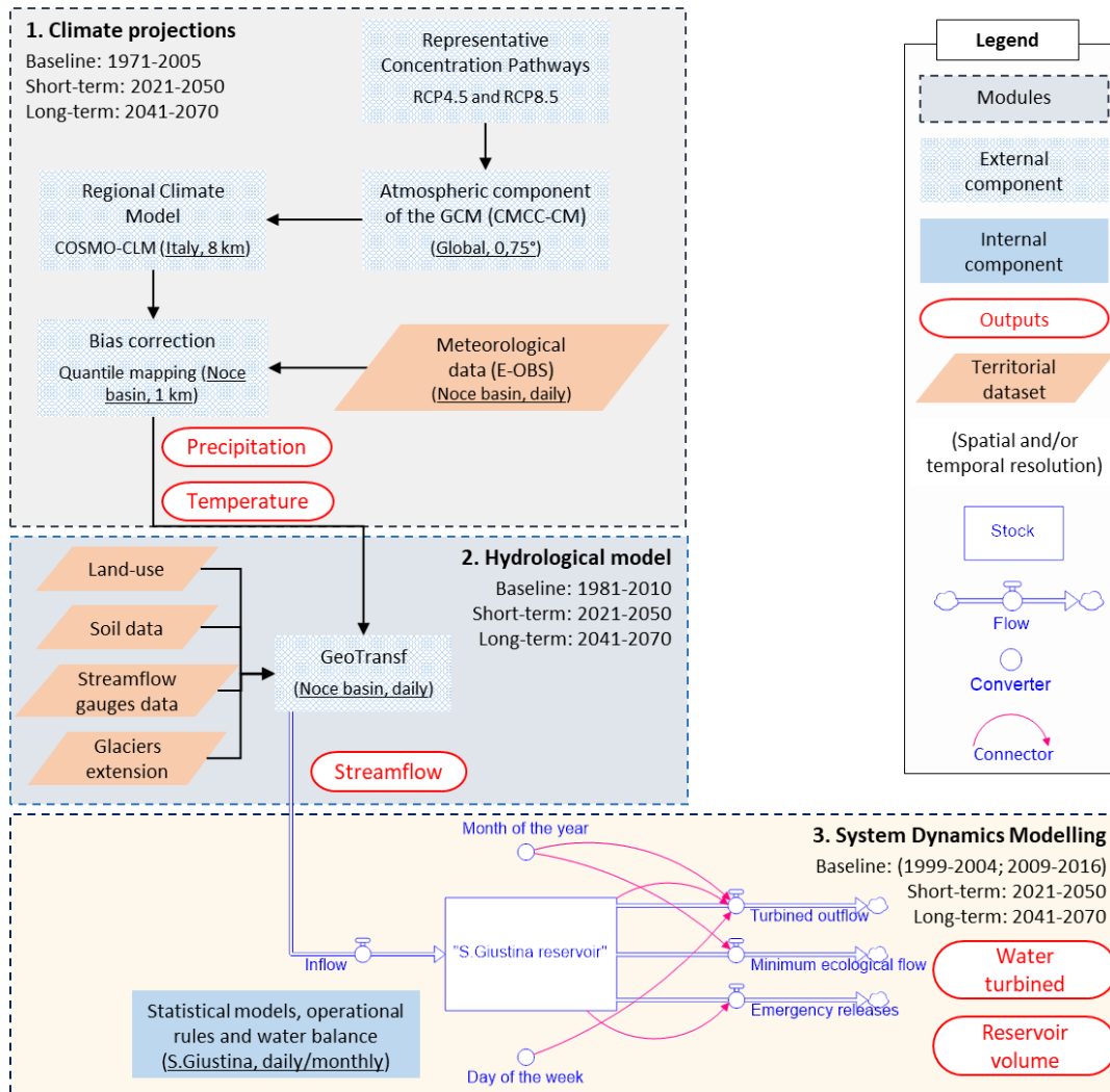
150 Figure 2 - Models' chain considered in this study. Box 1 includes the climate modelling used as input for the hydrological model simulation of water streamflow in box 2. Box 3 contains the SDM components of stock (S.Giustina reservoir), flows (inflow and three outflows), converters (month of the year, day of the week) and connectors (red arrows) considered to simulate stored water in the reservoir and the turbined outflow for hydropower production considering a baseline from 1999 to 2016 with a data gap from 2005 to 2008. Sources: adapted from Pham et al., 2018; Ronco et al., 2017. For interpretation of the references to colour in this figure legend, the reader is referred to the web version of this article.
