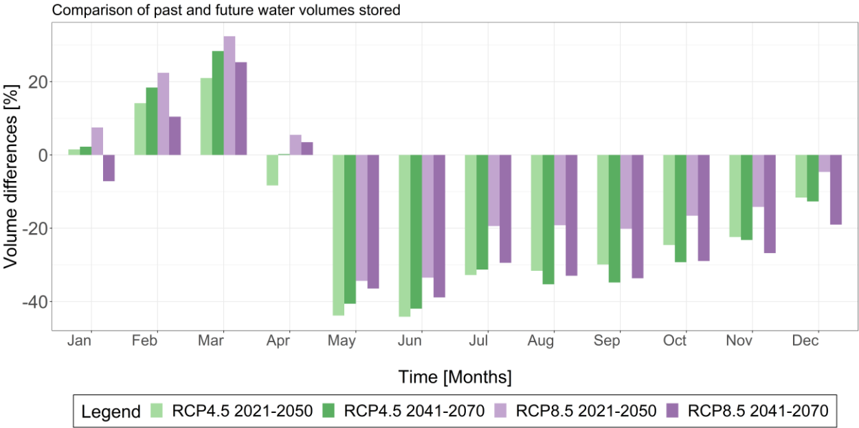
370 Figure 7 - Percentage change of volume [%] comparing the 4 climate scenarios to the baseline at monthly level
