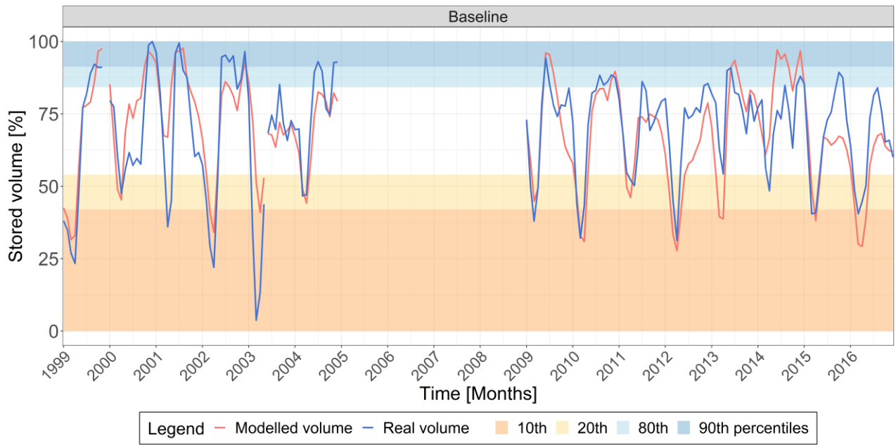
Figure 4 - S.Giustina stored volume values from 1999 to 2016, modelled values (red line) and real (blue line). Adjusted-R 2 = 0.60, RMSE= 19.74 Mm3. Coloured bands outline areas of values lower than the 10 th , 20 th and greater than the 80 th and 90 th percentiles.
