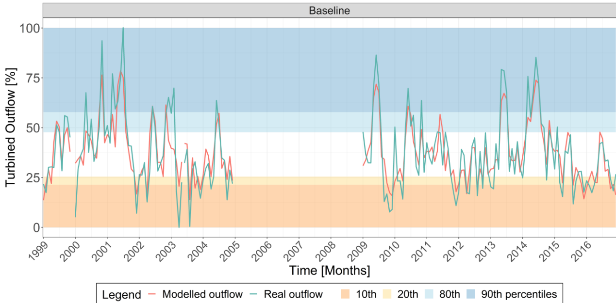
300 Figure 3 - S.Giustina water diverted to the turbines from 1999 to 2016. Modelled values (red line) and real (green line). Adjusted- R^2 = 0.75 , mean RMSE= 16.57 \text{ Mm}^3 . Coloured bands outline areas of values lower than the 10 th , 20 th and greater than the 80 th and 90 th percentiles.
