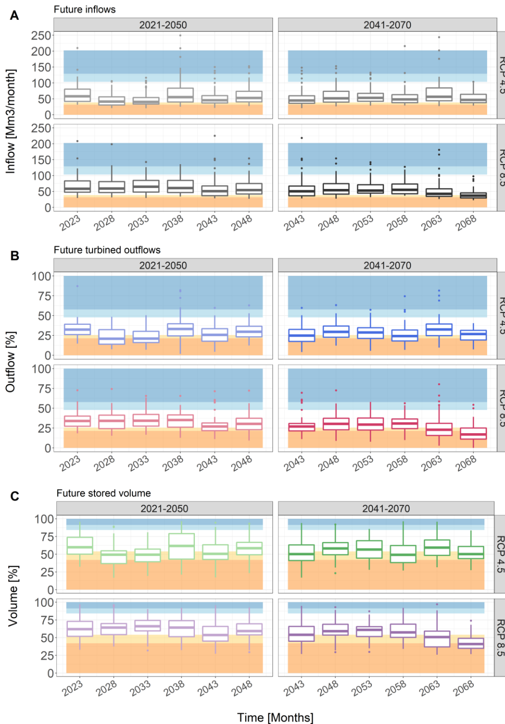
Figure 5 - 5-years slice boxplots for future projections of: A simulated water inflow to the S.Giustina reservoir, B simulated water turbined and C simulated future water volume stored in the S.Giustina reservoir. . Coloured bands outline areas of baseline values lower than the 10 th , 20 th and greater than the 80 th and 90 th percentiles.
