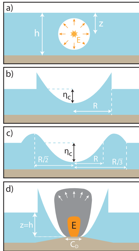
Figure 1 Illustrations of the submarine explosion problem. (a) An explosion of yield E at depth z in water of depth h . (b) The initial surface elevation profile is given by Eq. (1). (c) The initial surface elevation profile is given by Eq. (2). (d) Schematic of a volcanic scenario where such an explosion would occur at maximum depth where z = h , and crater diameter C_D can be measured or calculated using estimated ejecta volume V with Eqs. (9-10).
