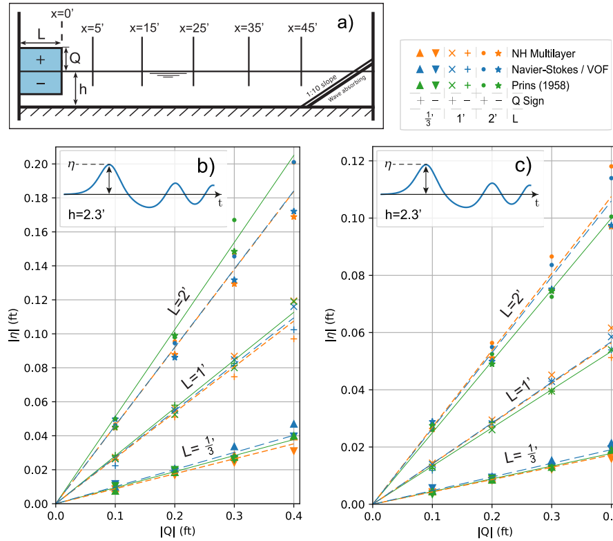
Figure 2. (a) Schematic diagram of Prins (1958) experimental set up, with gauge locations and the initial disturbance. (b) \eta - Q relation for first arrival crest or trough amplitude at x = 5 feet. (c) \eta - Q relation for first arrival crest or trough amplitude at x = 25 feet. Regression lines through origin are plotted for each L -model combination.
