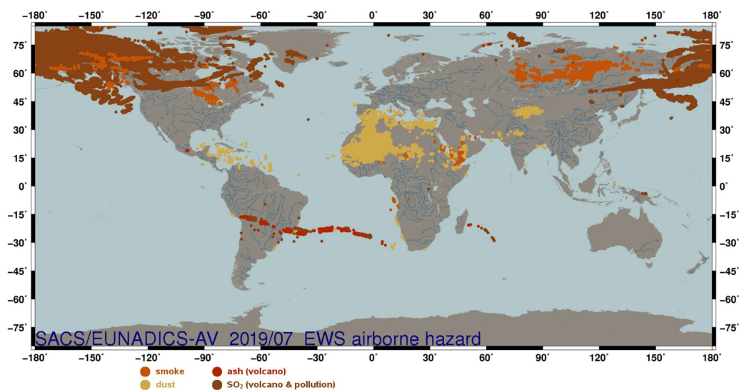
Figure 27: Selective detections of natural airborne hazards from EUNADICS EWS in July 2019 (Raikoke and Ubinas volcanic eruption, dust storms in Sahara and Gobi deserts, and forest fires in Russia and Canada).
