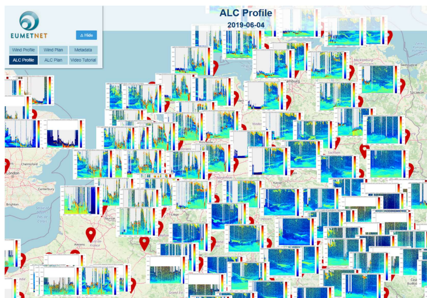
5 535 6 Figure 14: The E-PROFILE ALC network with quicklooks of attenuated backscatter observations from https://e-profile.eu . The quicklooks have time (0:00-24:00 UTC) on their x- and altitude above sea level (0-12 km) on their y-axis. The high values of attenuated backscatter correspond to clouds (orange and red) and aerosols (light blue, green and yellow). Low and mid-level clouds usually completely attenuate the signal above so that no observations above can be reported what is seen by the white areas in the quicklooks.
