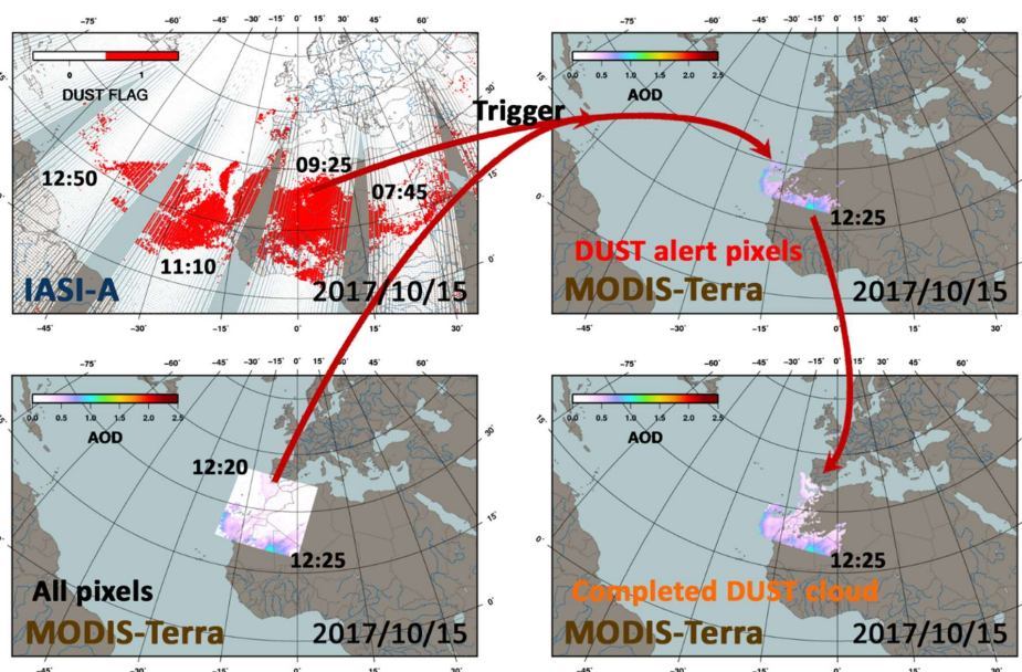
490 Figure 10: Illustration of the triggered approach to isolate MODIS-Terra AOD pixels related to desert dust (2017/10/15) using dust flag from IASI-A. Completed AOD data related to the dust cloud can be retrieved.
