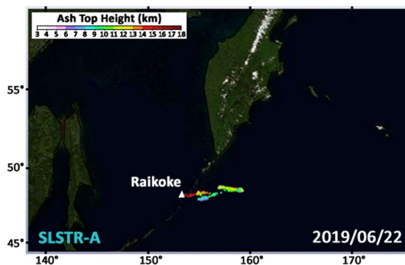
Figure 5: Characterisation of Raikoke plume by Ash Top Height (in km) from SLSTR-A on 22 June 2019.
