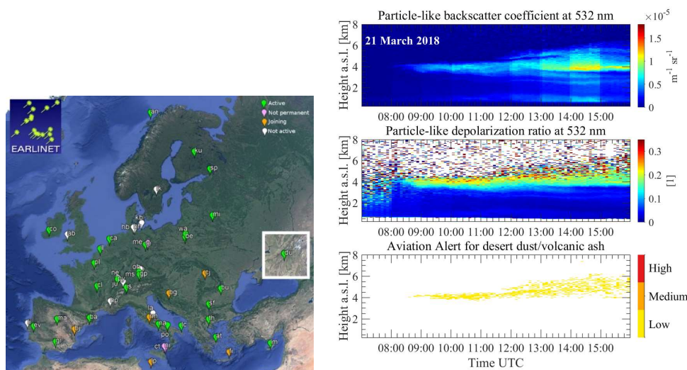
515 Figure 13: (left) Map of EARLINET network (from https://www.earlinet.org ), and (right) illustration of desert dust / volcanic ash alerts (station Finokalia) during desert dust storm on 21 March 2018 (particle backscatter coefficient at 532 nm, particle depolarization ratio at 532 nm, and alert for aviation.
