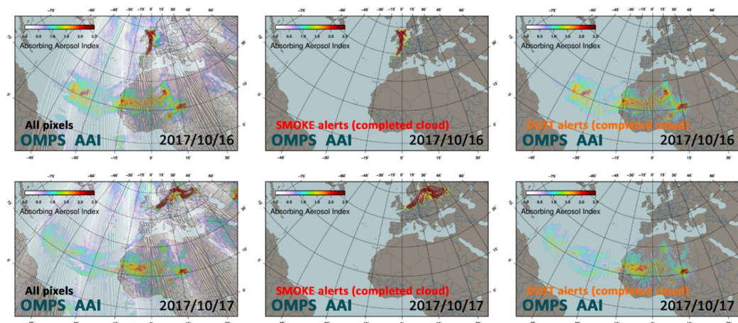
Figure 12: Isolated OMPS AAI pixels related to dust and smoke on 2017/10/16 and 2017/10/17.
