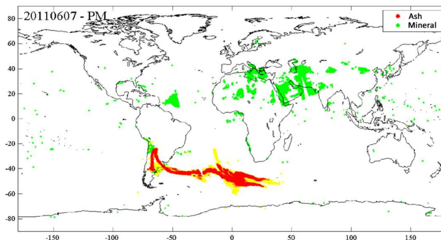
465 Figure 8: IASI-A detection of volcanic ash (Puyehue-Cordón Caulle eruption) and mineral dusts (windblown desert sands) on 7 June 2011 (afternoon).
