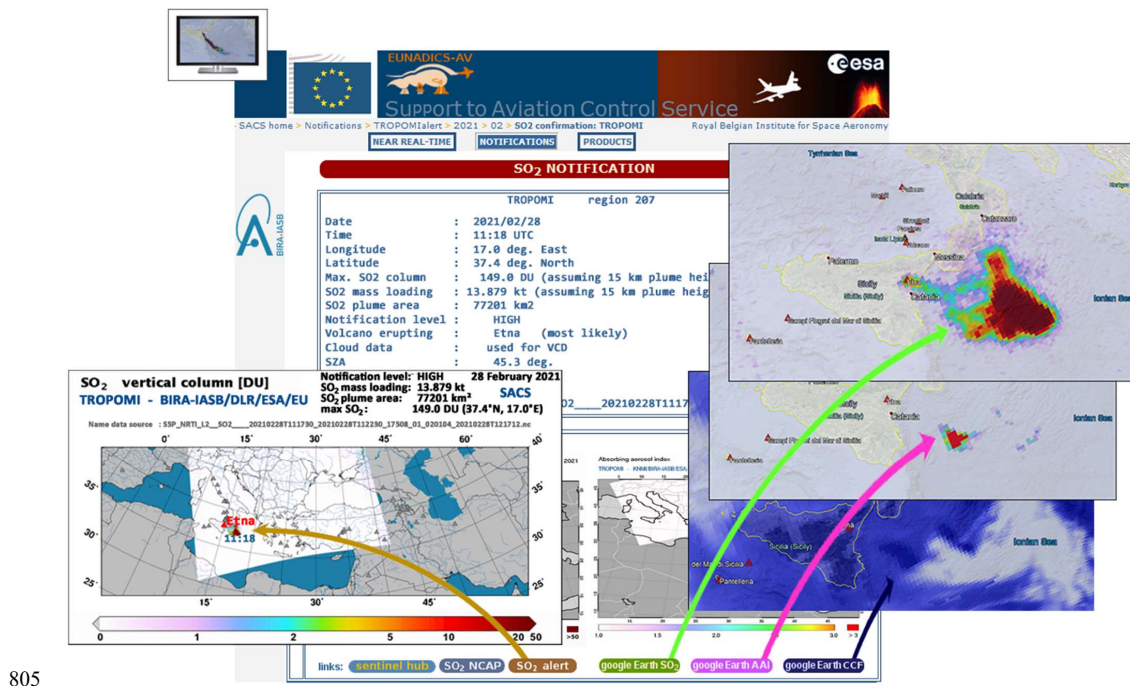
Figure 25: Example of alert webpage with illustration of visualisations offer for a paroxysm at Etna on 28 February 2021, i.e. notification information, SO 2 alert image, and SO 2 , Aerosol Absorbing Index (AAI) and Cloud Cover Fraction (CCF) © Google Earth images.
