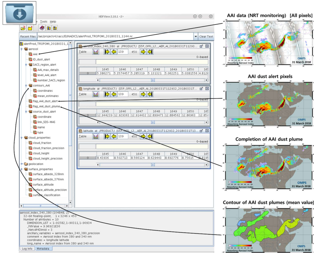
Figure 26: Illustration about the content of a NetCDF Alert Product (NCAP) file related to the Saharan sandstorm detection from OMPS on 31 March 2018.
