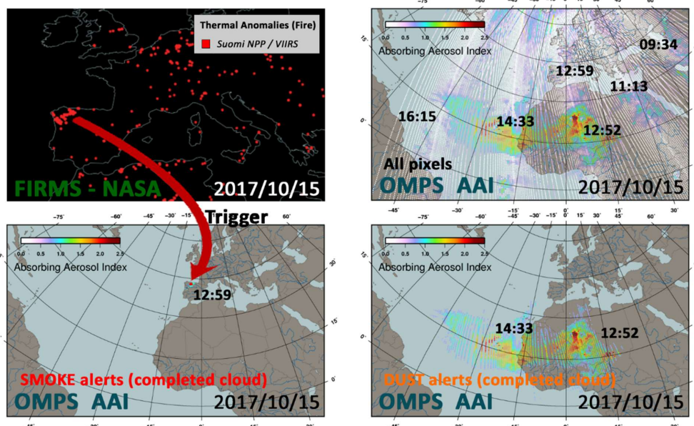
Figure 11: Illustration of the triggered approach to isolate OMPS AAI pixels related to smoke and dust (2017/10/15).
