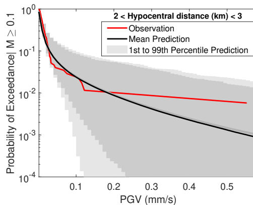
Figure 7. Validating the assumption of spatial correlation in the ground motions of the case study: Comparing predicted ground shaking with observed ground motion amplitudes. Also show in dark gray are the mean (solid line) and 1st to 99th percentile predictions (shaded area) for the base (uncorrelated) case.
