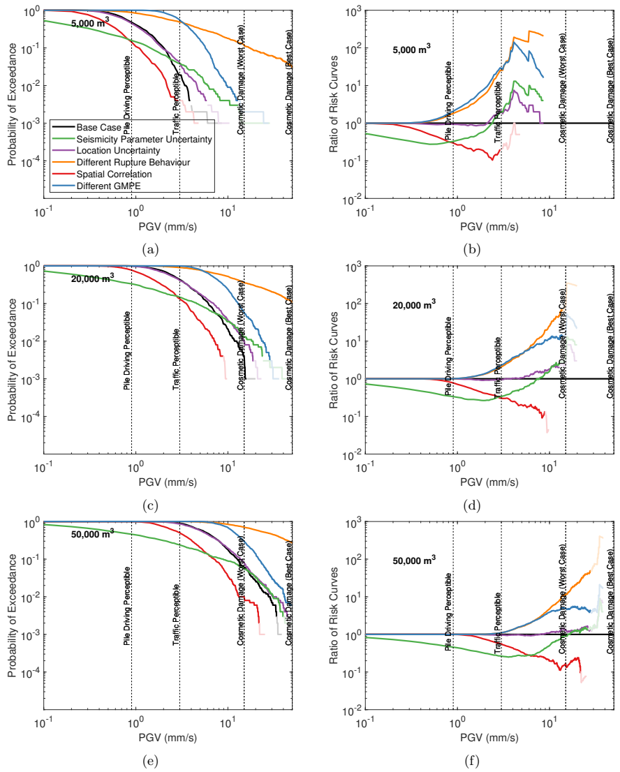
Figure 9. Quantifying the impact of alternative modelling assumptions on the probability of exceeding various PGV levels at least once across all considered buildings in the exposure model.
