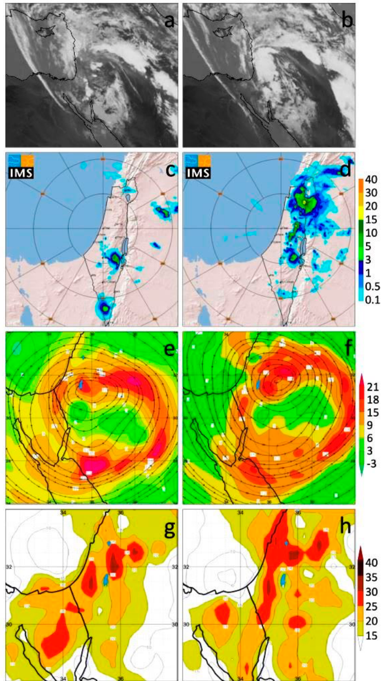
270 Figure 8: April 26 imageries for 09 (a,c,e,g) and 12 UTC (b,d,f,h) corresponding to the major rain centres including MSG IR images (a,b), one hour forward integration Radar [ \text{mm h}^{-1} ] images (c,d), relative vorticity [ \text{s}^{-1} \times 10^5 ] and streamlines at 500 hPa (e,f), and MKI [ ^{\circ}\text{C} ] (g,h). Panels e-f are based on ERA5 data at 30 km spatial resolution.
