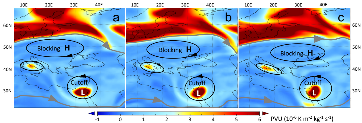
200 Fig. 5: PV distribution on 300 hPa, starting from April 25 2018, 12 UTC, in 6 hour intervals, covering Europe and the Mediterranean Basin, on which a conceptual sketch of a dipole type block (following Yamazaki and Itoh, 2013) is superposed. A cutoff low is seen over the south-eastern Mediterranean and a blocking high over Eastern Europe, forming a dipole. The arrows show the induced flow of each of the vortices.
