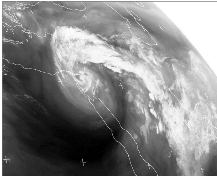
Figure 7: Water Vapor channel 6 (6.85–7.85 \mu\text{m} ) imagery of METEOSAT from April 25, 2018 21 UTC showing the cloud strip entering Israel from the east and the vortex over the south-eastern Mediterranean.
