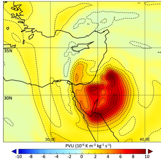
185 Figure 4: Potential Vorticity (PVU) at 300 hPa for April 26 00 UTC, taken from ERA-5, at 30 km spatial resolution. The major feature is a closed positive anomaly (with maximum of \text{K m}^2 \text{Kg}^{-1} \text{s}^{-1} ), corresponding to a cutoff low, centred over north-western Saudi Arabia.
