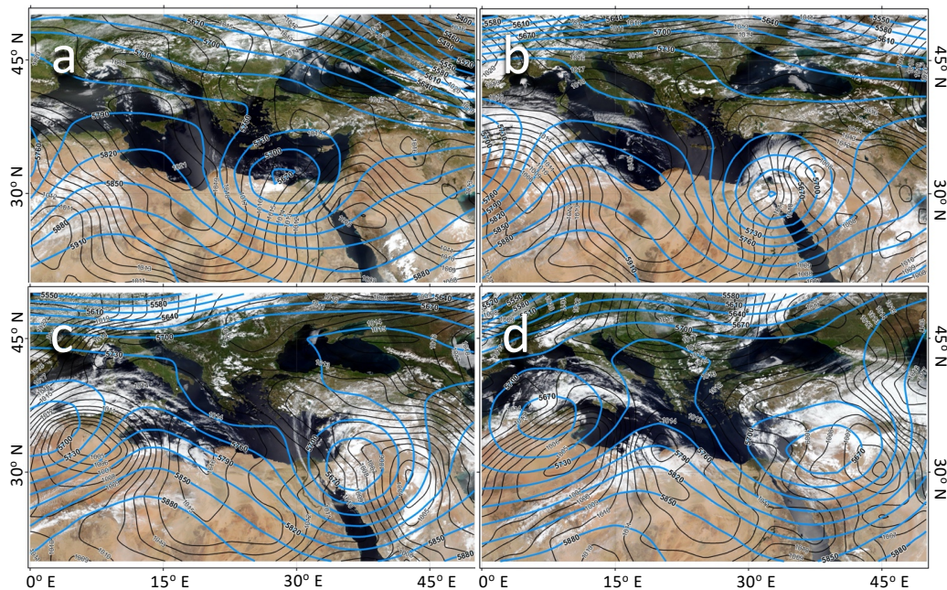
Figure 2: Geopotential height (GPH) at 500 hPa (m) and SLP (hPa) projected on MODIS imagery, in 24 h intervals, for April 24–27 2018, 12UTC (a–d, respectively).
