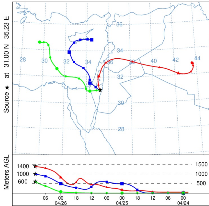
Figure 6: Sixty hours back-trajectory of the air arriving at Tzafit Basin at April 26, 2018 10 UTC at heights 600, 1000 and 1400 m.
