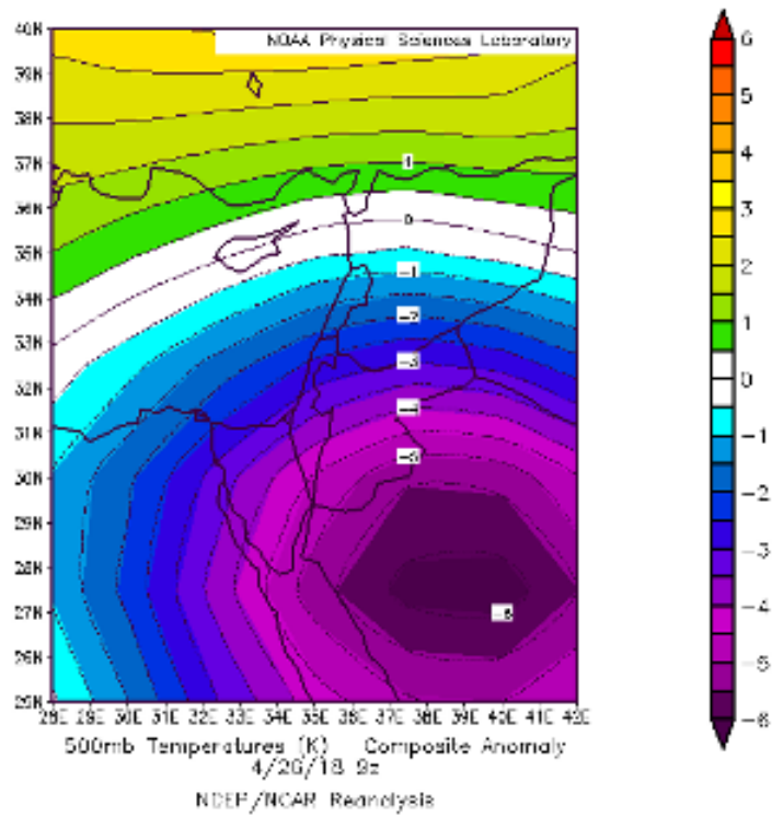
Fig. 7. temperature anomaly at 26 April 2018, 09 UTC.
