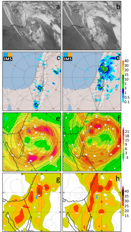
Fig. 4. Set of maps for April 26 2018, 09 and 12 UTC: Satellite image of MSG ch9 (10.8 um) (a,b); Radar imagery of one hour integrated rain depth (mm), (c,d); Relative vorticity and wind (e,f) and MKI (g,h).
