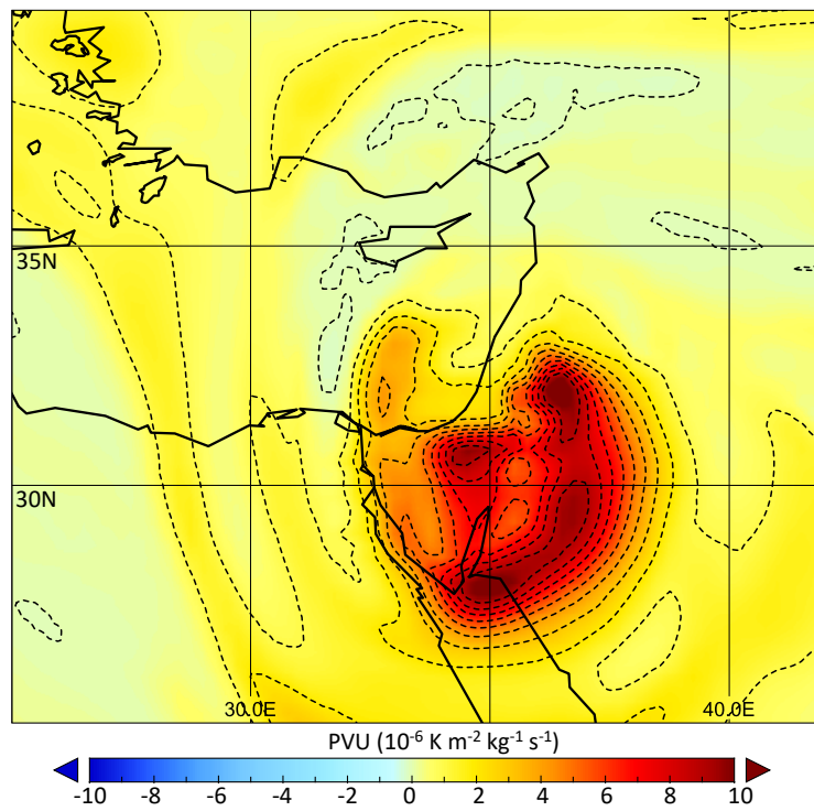
Fig. 5. PVU and enlarged domain of org Fig. 4.
