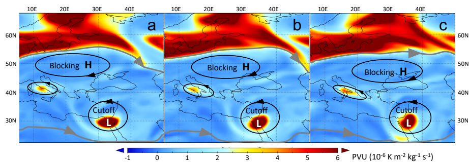
Fig. 1. PV distribution on 300 hPa, starting from April 25, 2018, 12 UTC, in 6-hour intervals, covering Europe and the Mediterranean Basin, on which a conceptual diagram of a dipole type block (following Yama
