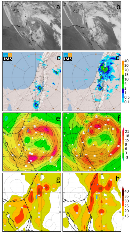
Fig. 2. Fig. 5. Set of maps for April 26 2018, 09 and 12 UTC: Satellite image of MSG ch9 (10.8 um) (a,b); Radar imagery of one hour integrated rain depth (mm), (c,d); Relative vorticity and wind (e,f) and MKI
