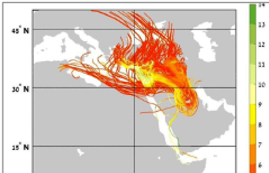
Fig. 3. Air back-trajectories arriving at Tzafit (31.1N, 35.2E) in 26 April 2018 09 UTC. The colors denote specific humidity along the trajectory (g/Kg).
