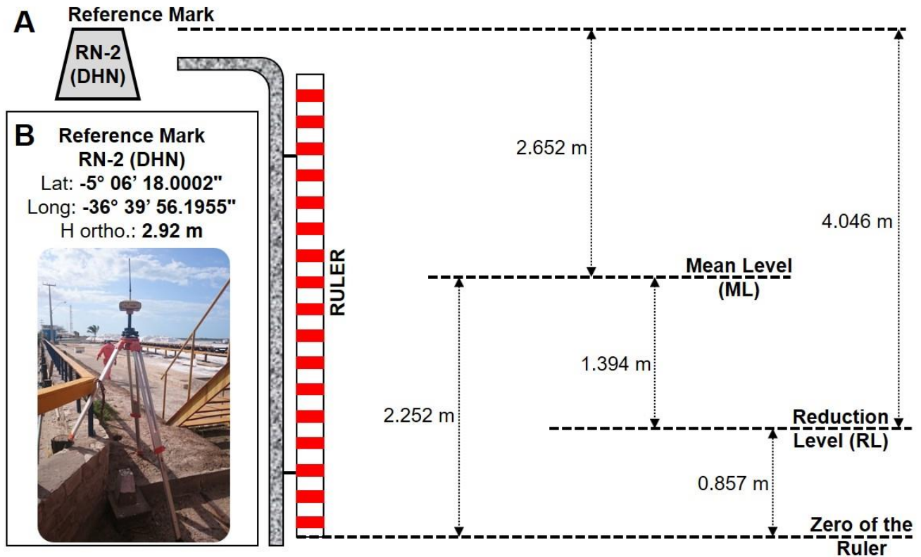
535 Figure 3: Scheme illustrating the differences in quotas between the references adopted by the Brazilian Navy: (A) Reference Mark RN-2 (DHN); and (B) Coordinates of Reference Mark RN2- (DHN).
