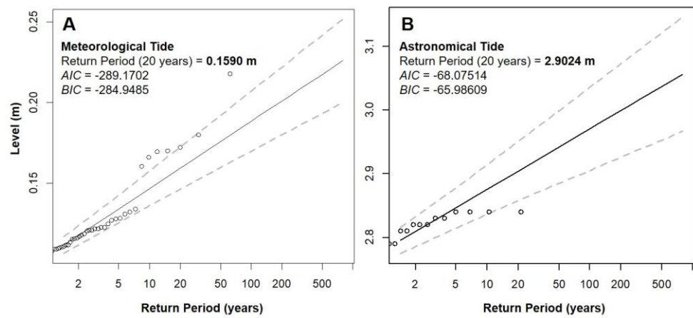
595 Figure 5: Return period graph of tide data: (A) Meteorological tide; and (B) Astronomical tide.
