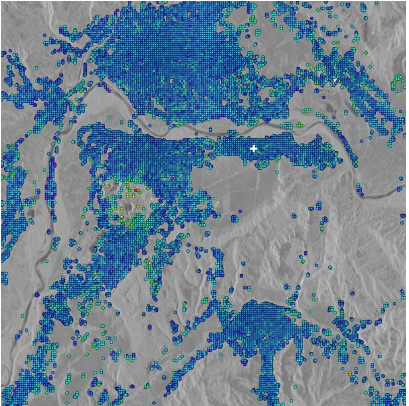
Supp. Fig. 1. LoS linear deformation rate from ascending Sentinel-1 scenes (track 29) in radar geometry, white cross shows non-deforming reference area. Same colorscale as Fig. 6. Contains modified Copernicus Sentinel data [2014-2019]
