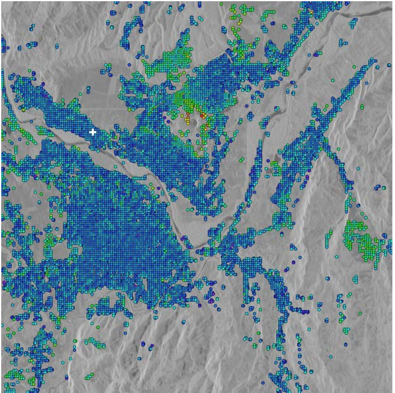
Supp. Fig. 2. LoS linear deformation rate in radar geometry determined from Sentinel-1 data of track 80 (descending pass), white cross shows non-deforming reference area. Same colorscale as Fig. 7. Contains modified Copernicus Sentinel data [2014-2019]
