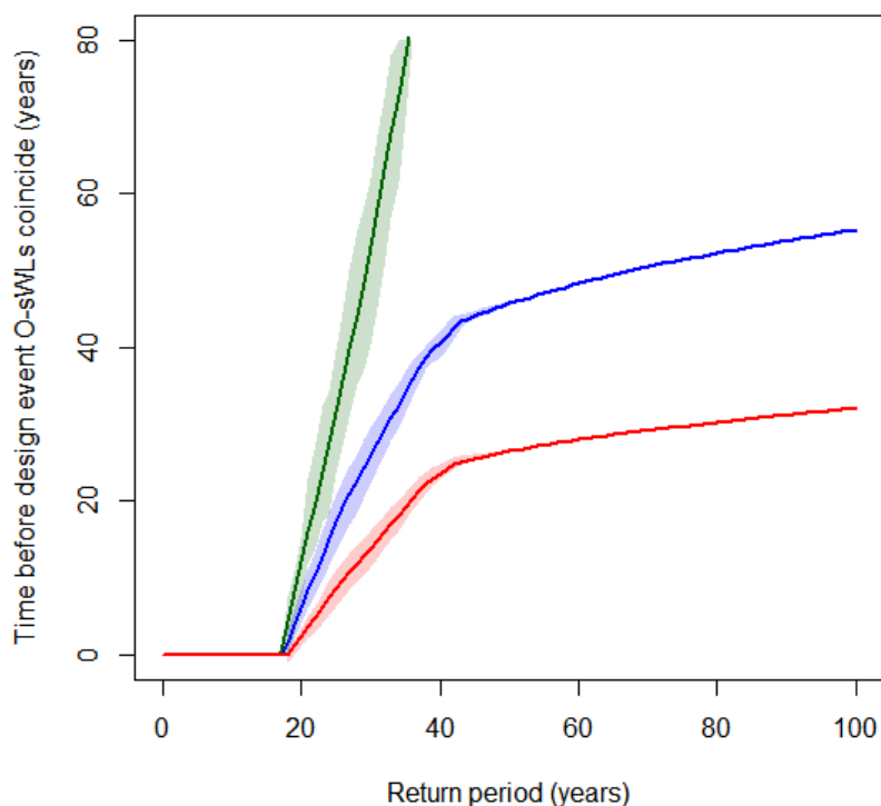
Figure 7: Time before the O-sWL in the bivariate design event derived from the two-sided sampling approach reaches corresponding value obtained from the original design approach (i.e., full dependence assumption) under the low (green), intermediate (blue), and high (red) SLR scenarios given in Sweet et al. (2017). Shaded regions denote 95% (basic) bootstrap confidence intervals.
