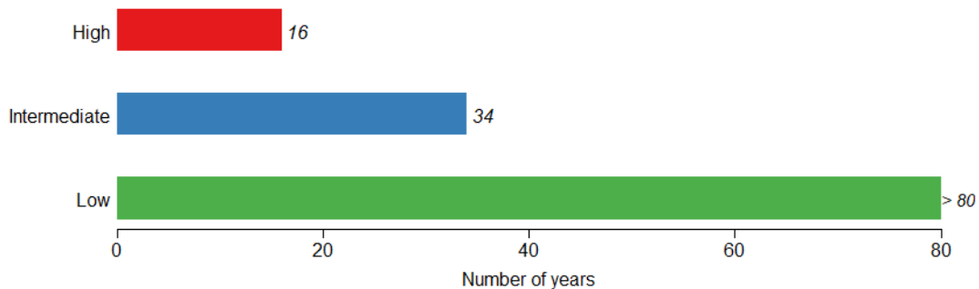
460 Figure 6: Top: Regional SLR projections for Miami Beach given in Sweet et al. (2017). Bottom: Number of years before the O-sWL in the 50-year design event derived using the bivariate approach reaches the corresponding value obtained using the original design approach according to the three SLR scenarios.
