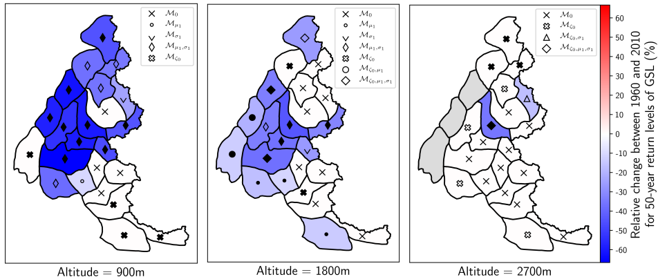
Figure 5. Trends in 50-year return levels of ground snow load (GSL) between 1960 and 2010 at low (900 m), mid (1800 m) or high (2700 m) altitude. Markers show selected model \mathcal{M}_N while filled markers symbolize models that are significantly better than the Gumbel model \mathcal{M}_0 (Sect. 4.2). Grey areas denote missing data, e.g. when the altitude considered is above the top altitude of the massif.
