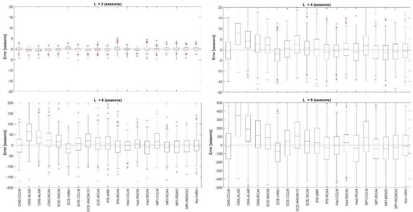
830 Figure 13. Box-plots representing the frequency distribution of RCMs percentage errors in the return period of drought event of duration L equal to 2, 4, 6 and 8 seasons.
