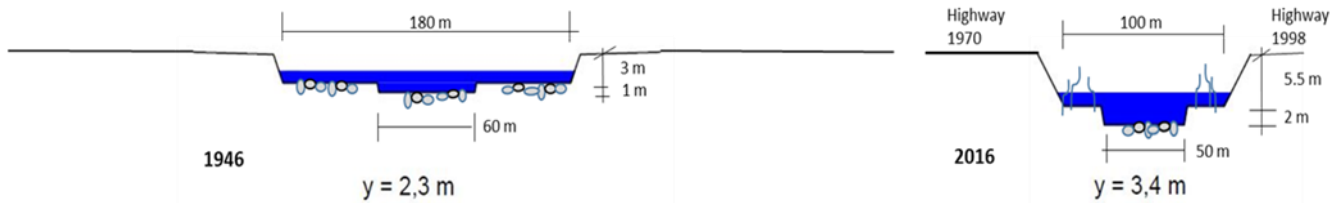
Fig.6. Cross-sections of reach 1 for the two extreme dates, 1946 (left) and 2016 (right). Alluvial widths are 175 m and 33 m respectively (table 3, later). Depth y drawn in the cross-sections corresponds to a discharge of 600 \text{ m}^3/\text{s} , within the first day of the flow duration curve.
