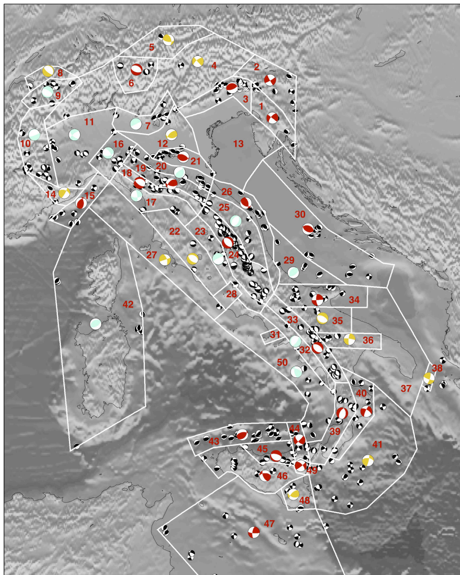
455 Figure 2 - Results of summation using a 20 km seismogenic layer thickness for all the seismic zones. Coloured focal mechanisms are the result of the summations: red ones represent stable cumulative focal mechanisms, yellow are less reliable ( low number of events to cumulate), light blue are unstable because of the heterogeneity of the input dataset. In the background: the entire available dataset in black; in white the seismic zones in ZS16 numbered in red.
