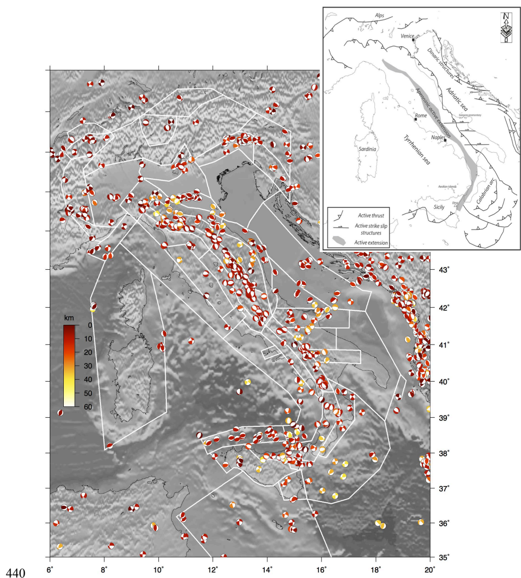
Figure 1 - Map of the entire dataset used for this study (see data in Table 1_SupplementaryMaterial). Different colors for the focal mechanisms represent different hypocentral depths, following the scale on the left. In the background, the borders of the seismic source zones in ZS16 are reported in white. Top right, a seismotectonic sketch of the study region.
