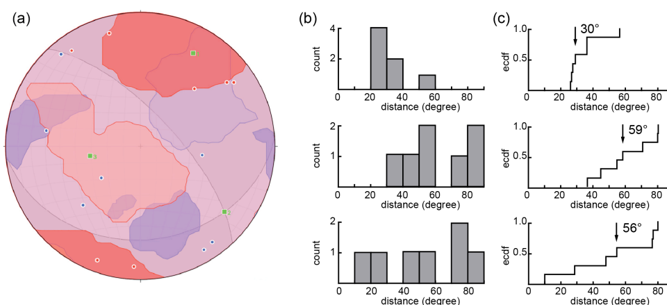
475 Figure 4 - Example of data dispersion analysis for the seismic zone n.9. On the left is drawn the possible cumulative focal mechanism obtained with the summation of all input data , all strike slip . On the right, the dispersion plots where P, T and B axes of the cumulative and the single input data are compared. The angular difference between P and T axes is greater than 30°, and the final solution is a strike slip, but random (see Table 1).
