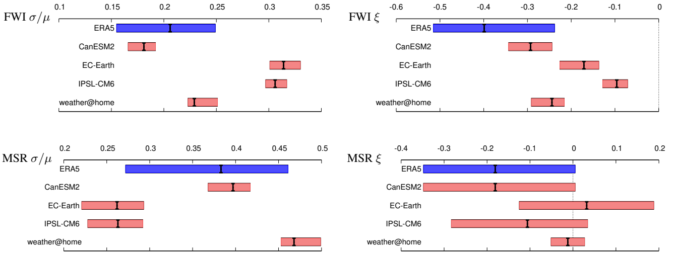
Figure 5. Model verification for FWI (top) MSR (bottom). The left figures show the dispersion parameter \sigma/\mu and the right figures the shape parameter \xi . The bars denote the 95% uncertainty ranges.
