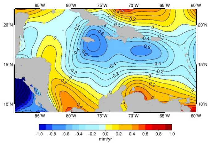
Figure 5: Sea level trends in the Caribbean basin (whereas the global mean trend 3.00 \pm 0.4\text{mm yr}^{-1} is removed), calculated using satellite altimetry data 1993-2018.
