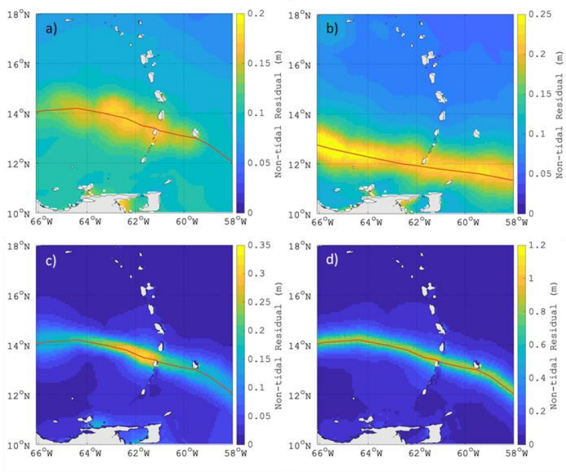
Figure 9: Maximum non-tidal residual envelopes for four model runs: a) ERA5-forced Hurricane Tomas, b) ERA5-forced Hurricane Ivan, c) Holland-forced Hurricane Tomas and d) 'Enhanced Tomas' case study.
