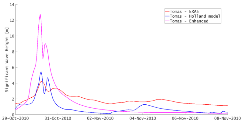
Figure 8: Significant wave height at Argyle airport during Hurricane Tomas: red line – wave model run forced with the ERA5 reanalysis; blue line – wave model forced with the Holland’s model parametric winds; pink line – wave model forced with “worst case scenario” enhanced winds.
