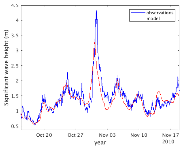
740 Figure 2: Time series showing a zoom to the dates of Hurricane Tomas (Oct 2010) from the global model and observations at the buoy 42060 (see Fig. 1 for location).
