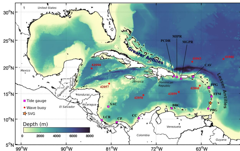
735 Figure 1: Map of the Caribbean Sea, showing bathymetry and locations of 12 tide gauges and 7 wave buoys used for models validation. Tables SI2 and SI3 give the locations of the tide gauges and wave buoys respectively.
