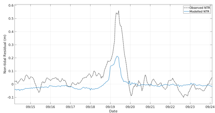
745 Figure 3: Modelled and observed non-tidal residuals (m) during the passing of Hurricane Maria (2017) over the Port-au-Prince tide gauge (Port-au-Prince, Guadeloupe).
