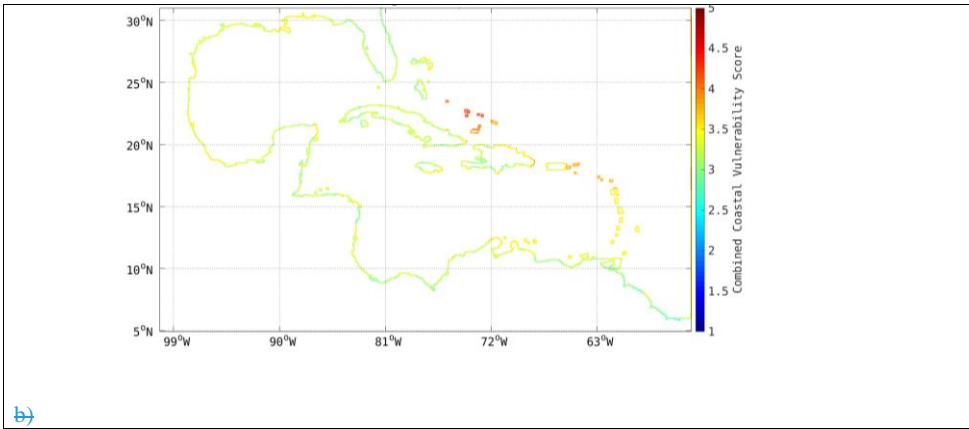
Figure 10: Coastal vulnerability metrics; a) combined based on mean annual rate of sea level rise, mean wave height and Great Diurnal Tidal Range and b) as a) plus maximum windspeed
