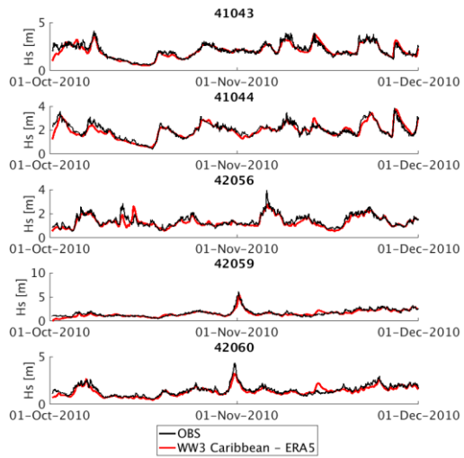
Figure 4: Comparison between the significant wave heights observed by 5 buoys from the NOAA National Data Buoy Center and modelled by the WW3 Caribbean model forced by ERA5 reanalysis winds. Validation is for October 2010 and November 2010, covering the passage of Hurricane Tomas (29 October 2010 – 14 November 2010).
