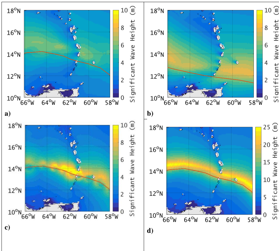
Figure 7: Maximum significant wave height simulated by the WW3 Caribbean model during a) Hurricane Tomas (2010) and b) Hurricane Ivan (2004) forced by ERA5 and c) Hurricane Tomas (2010) forced by the Holland model parametric wind field and d) Hurricane Tomas (2010) forced by the enhanced wind field.
