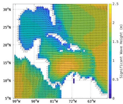
Figure 6: Mean significant wave height (m, colour shading) and mean direction (vectors) from the global 37-year historic climatology wave model run.
