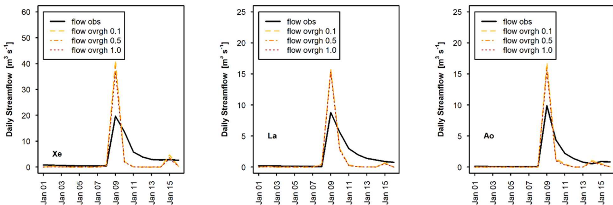
Figure 4. Hydrographs obtained at three different watersheds for OVRGH values of 0.1 (flow ovrg 0.1), 0.5 (flow ovrg 0.5), and 1.0 (flow ovrg 1.0), in comparison to observed flow (flow obs). For watershed short names refer to Table 1.
