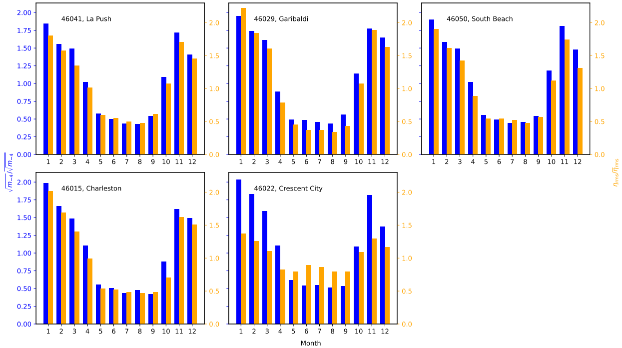
Figure 17. Monthly \sqrt{m-4}f_{m2}/\sqrt{m_0} (blue) from ocean wave spectra and \eta_{rms}/\eta_{rms} (orange) at the tide gages, computed from 0.5-hour window, for year 2016.
