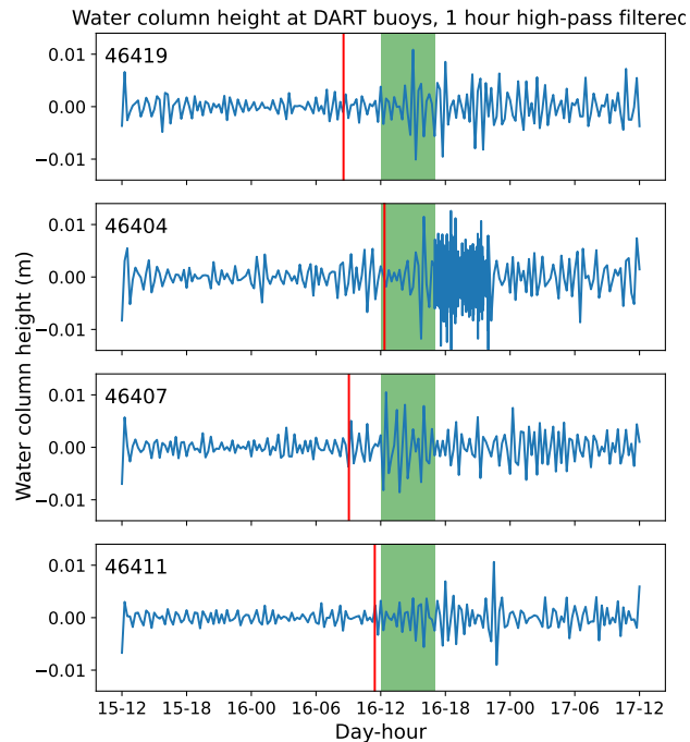
Figure 10. Water column height deviations (1-hour high-pass filtered) at DART sensors from January 15, 12:00 – January 17, 12:00, 2016. Red vertical lines represent January 16, 8:00 , 33, 12:21 , 9:03 , and 11.27 , respectively from top to bottom, i.e. the approximate onset of unusual water level fluctuations at the tide gages. Green bars indicate time period during which videos of large runup and injury reports took place, i.e. between January 16 12:00 to January 16 17:00. Between approximately January 16 17:00 to January 16 22:00, the 46404 station was in higher sampling mode.
