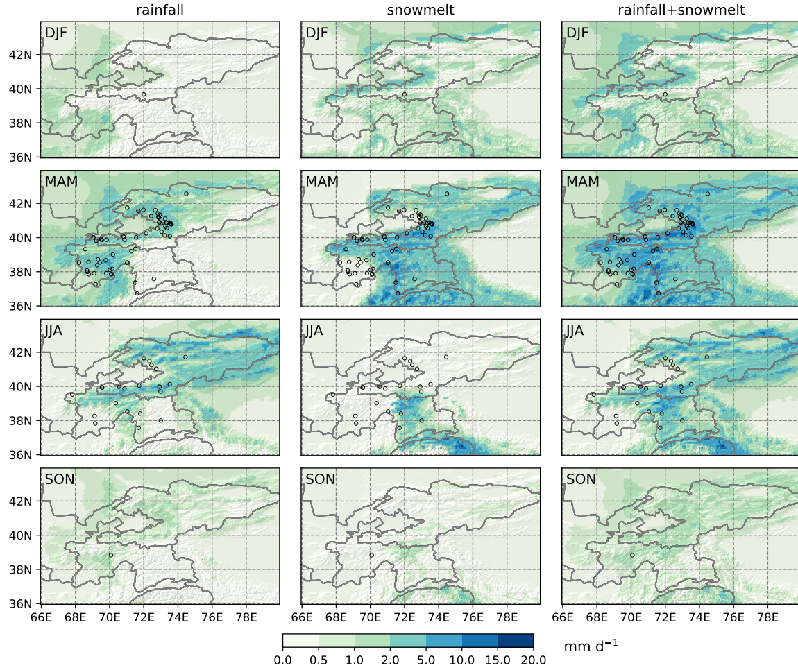
Figure 2. Seasonal rainfall, snowmelt, and rainfall+snowmelt from the HAR v2 from 2004-2018. Black circles: seasonal landslide events from GLC and GFLD. Topographic shading is based on DEM data from SRTM. DJF: December-February; MAM: March-May; JJA: June-August; SON: September-November.
