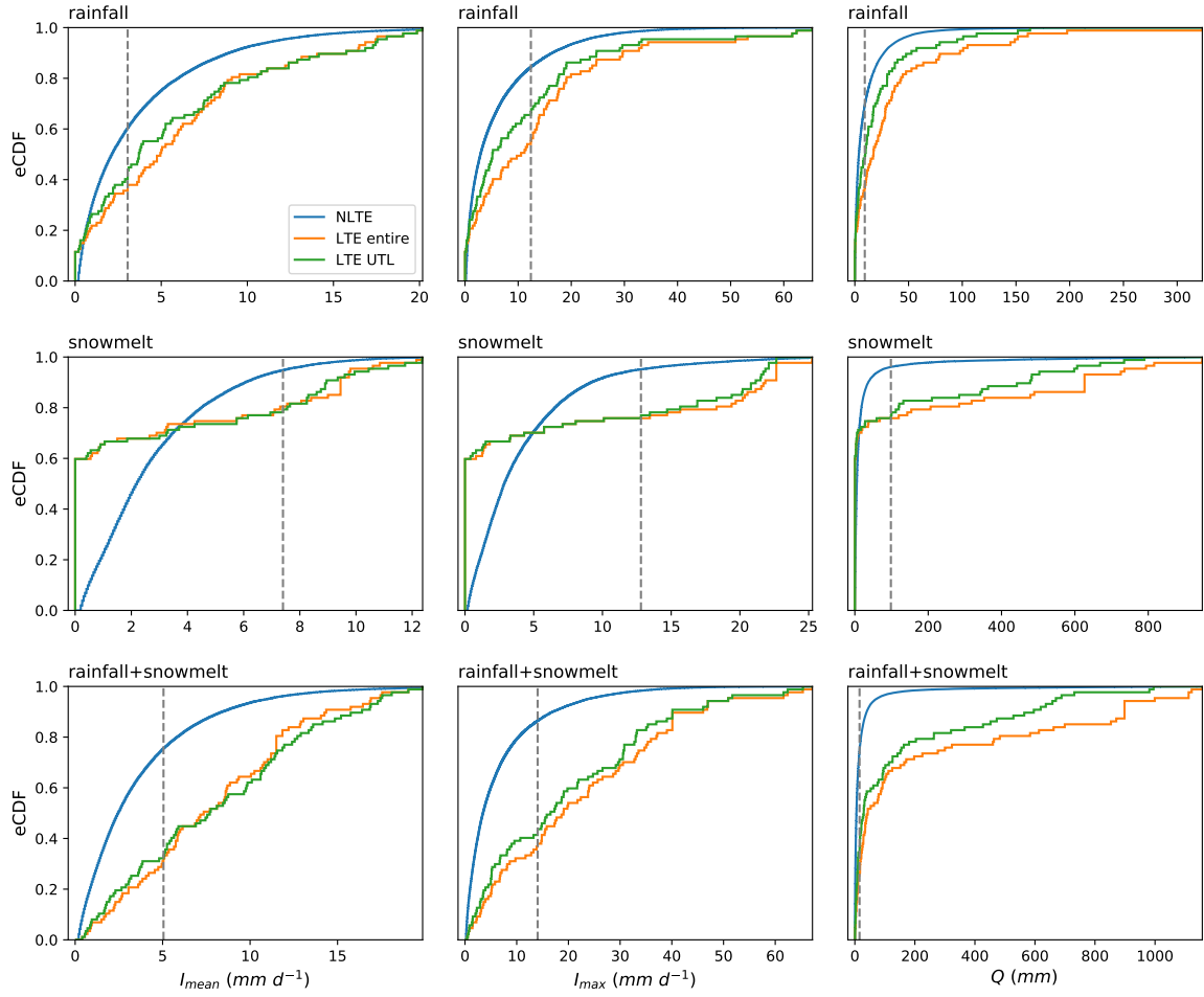
Figure 5. eCDF curves of I_{mean} , I_{max} , Q of NLTE, landslide-triggering entire event (LTE entire), and landslide-triggering up-to-landslide event (LTE UTL) for rainfall, snowmelt, and rainfall+snowmelt during the period of 2004–2018. Grey dashed lines represent the thresholds for UTL event defined in Table 1.
