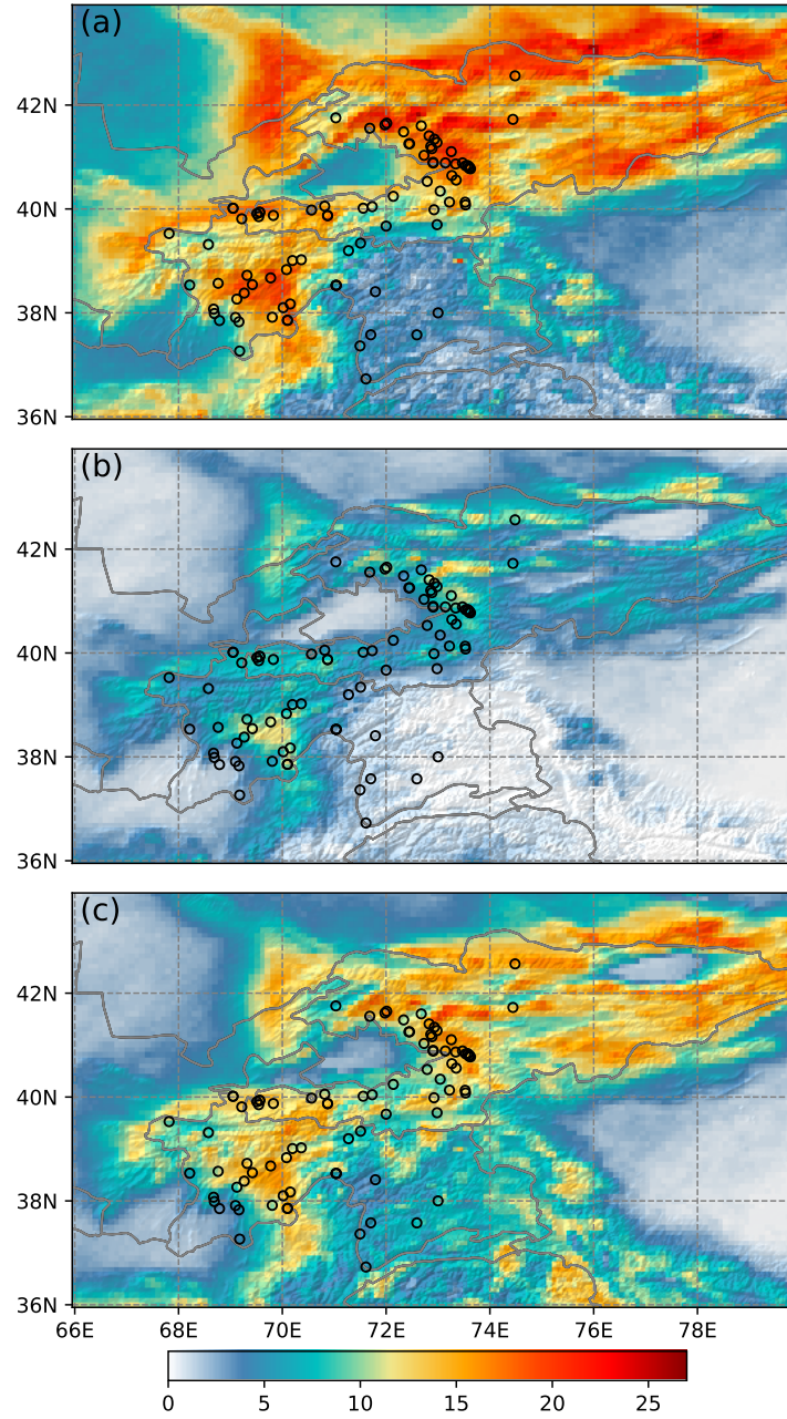
Figure 6. Mean annual exceedance (number of events per year) of (a) I_{mean} = 5.05 \text{ mm d}^{-1} (b) I_{max} = 14.05 \text{ mm d}^{-1} ; and (c) Q = 15.65 \text{ mm} for the rainfl+snowmelt UTL events. Black circles: landslide events from GLC and GFLD. Topographic shading is based on DEM data from SRTM.
