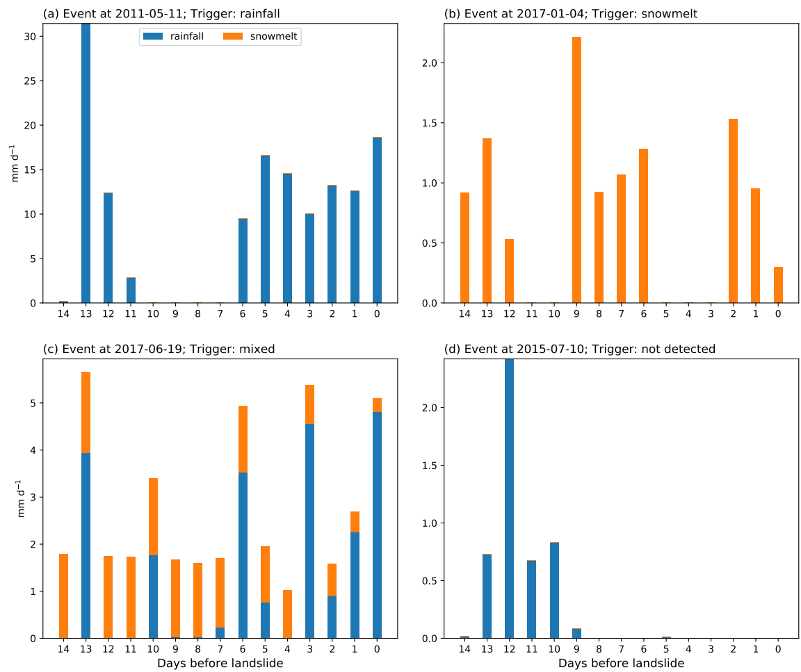
Figure A1. Event-based temporal process of rainfall and snowmelt for selected landslide events with landslide triggers defined as (a) “rain-fall”, (b) “snowmelt”; (c) “mixed”; and (d) “not detected” according to the method described in section 2.2.1.
