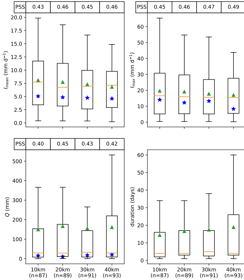
Figure 7. Boxplots demonstrating the impact of spatial resolution of atmospheric data on I_{mean} , I_{max} , Q , and duration of LTE UTL events, as well as the associated landslide triggering thresholds (blue stars). The yellow line denotes the median and the green triangle indicates the mean. Outliers are not shown for a better intercomparison. n denotes the number of landslide events detected by rainfall+snowmelt.
