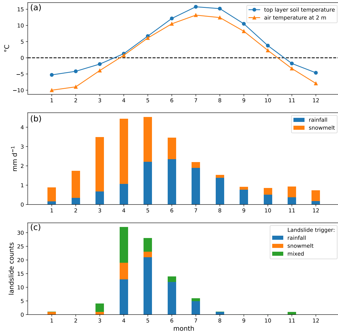
Figure 4. (a) Mean monthly soil temperature at the top soil layer (0-0.1m) and air temperature at 2 m averaged over Kyrgyzstan and Tajikistan extracted from the HAR v2; (b) mean monthly rainfall and snowmelt averaged over Kyrgyzstan and Tajikistan extracted from the HAR v2; (c) mean monthly landslide occurrences in Kyrgyzstan and Tajikistan from 2004-2018.
