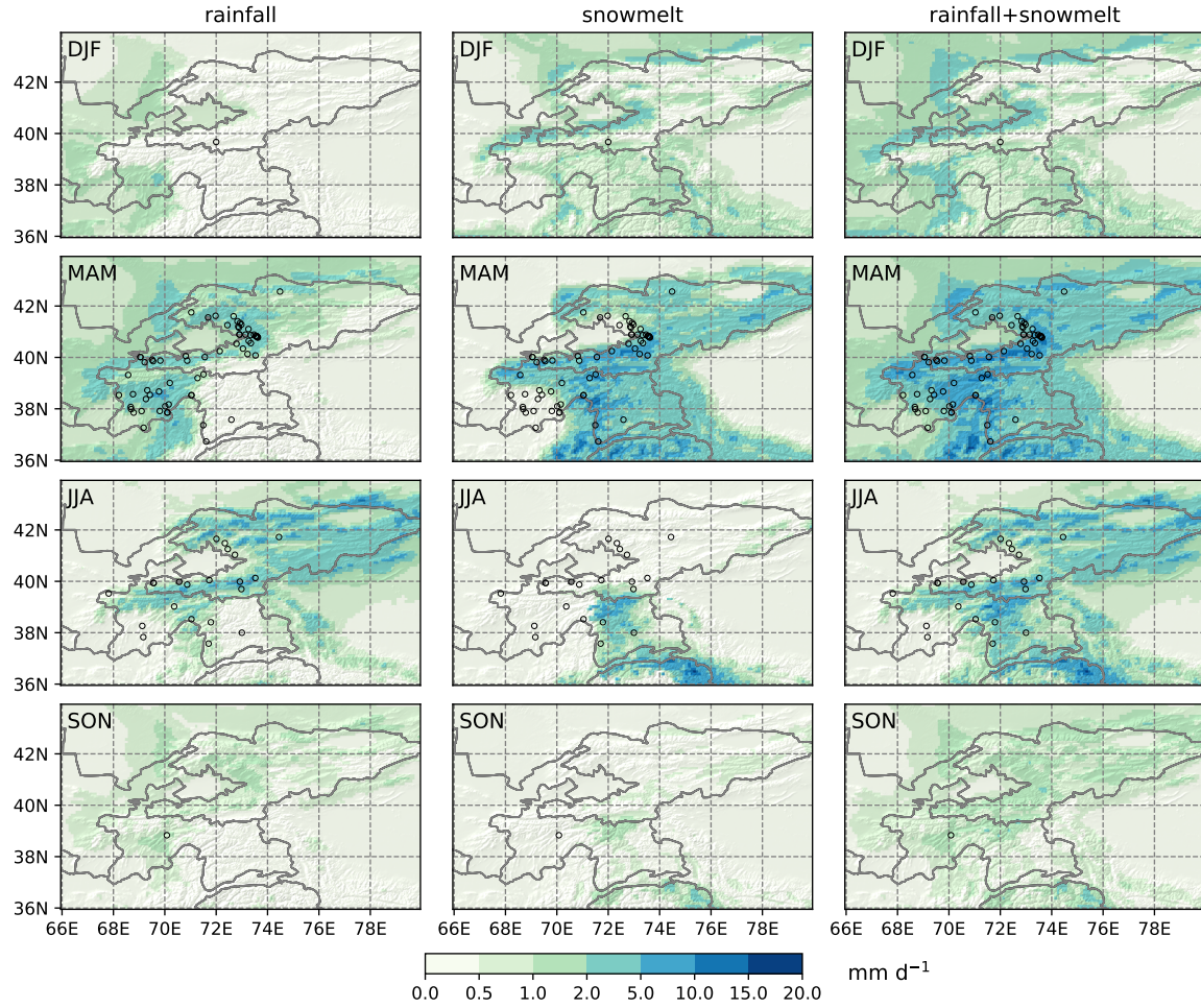
Figure 2. Seasonal rainfall, snowmelt, and rainfall+snowmelt from the HAR v2 from 2004-2018. Black circles: seasonal landslide events from GLC and GFLD. Topographic shading is based on DEM data from SRTM. DJF: December-February; MAM: March-May; JJA: June-August; SON: September-November.
