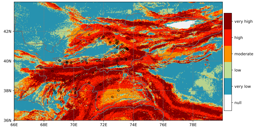
Figure 8. Non-climatic landslide susceptibility map computed using slope, geology, fault zones, road networks, and forest loss developed by Stanley and Kirschbaum (2017). Black circles: landslide events from GLC and GFLD. Topographic shading is based on DEM data from SRTM.
