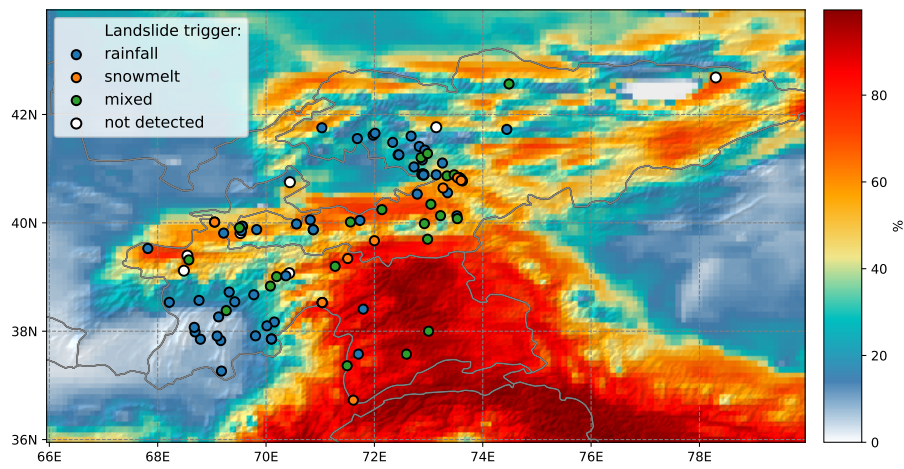
Figure 3. Contribution (%) of snowmelt to annual sum of rainfall and snowmelt (background contour) and climatic triggers of 96 landslide events extracted from GLC and GFLD (points). Topographic shading is based on DEM data from SRTM.
