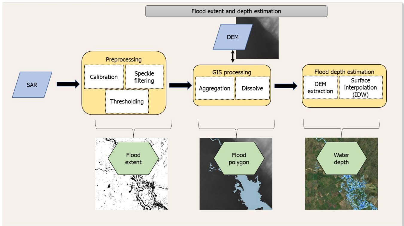
290 Figure 4: The workflow representing the extraction SAR satellite imagery and deriving its corresponding water depth. The flood polygon is shown on SRTM DEM and the water depth map is shown on © Google Satellite.
