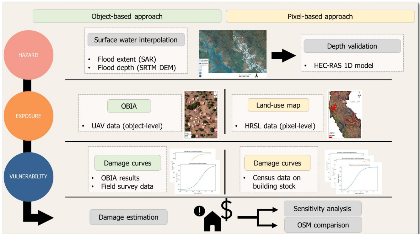
260 Figure 3: Workflow of the two approaches of flood damage estimation. The left panel shows the object-based approach, the right panel shows the pixel-based approach. Abbreviations: Synthetic-aperture radar (SAR), Shuttle Radar Topography Mission (SRTM) digital elevation model (DEM), Object-Based Image Analysis (OBIA), High-Resolution Settlement Layer (HRSL), OpenStreetMap (OSM). The inundation (hazard) map is shown on © Google Satellite. The OBIA and land-use map are created using UAV imagery from the Malawi Red Cross Society.
