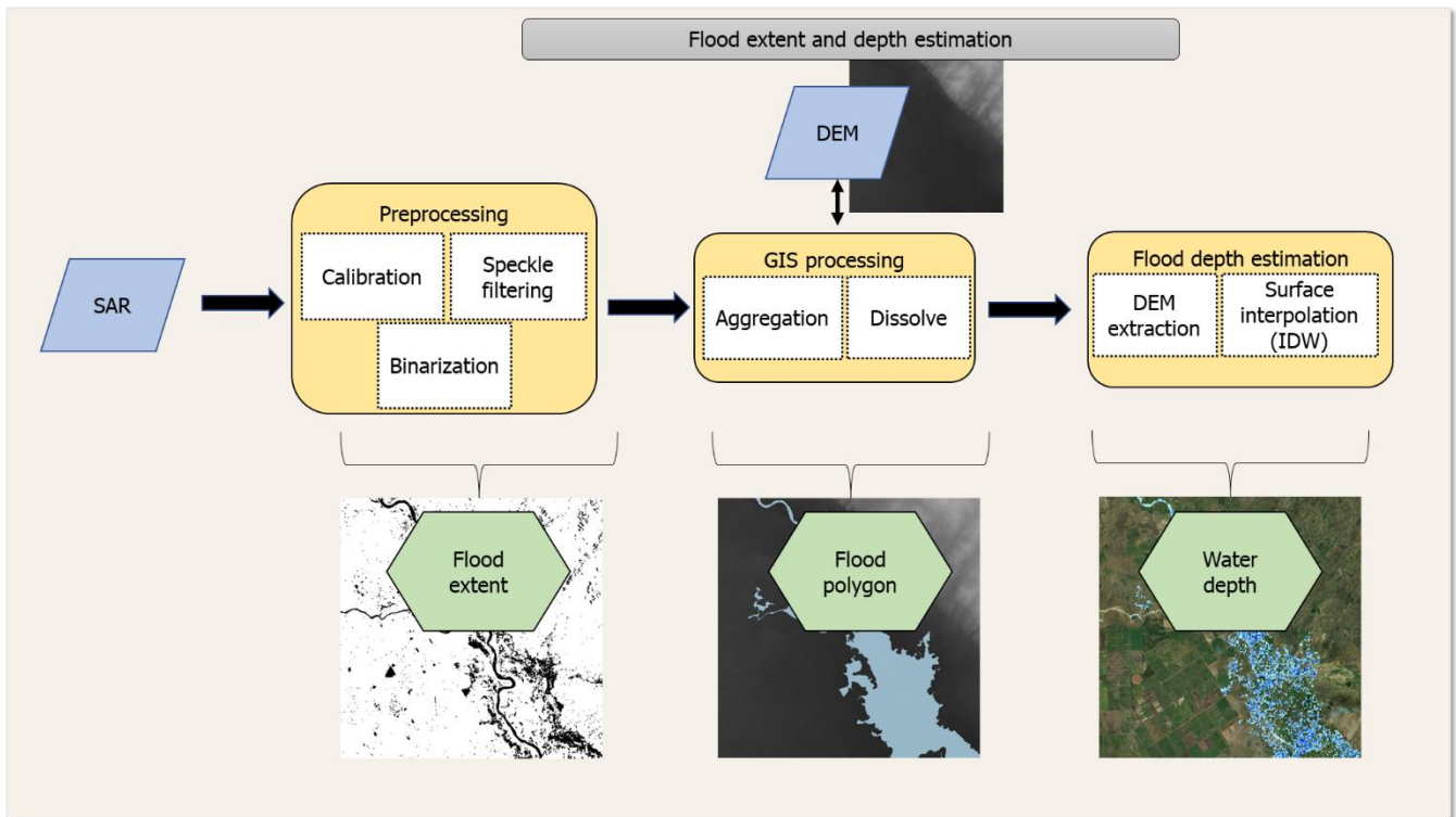
Figure 4.: the workflow representing the extraction SAR satellite imagery and deriving its corresponding water depth. The flood polygon is shown on SRTM DEM and the water depth map is shown on © Google Satellite.
