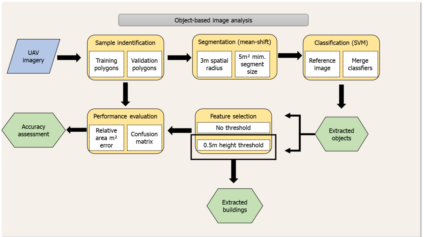
345 Figure 6: conceptual model of the building classification using automatic extraction methods.
