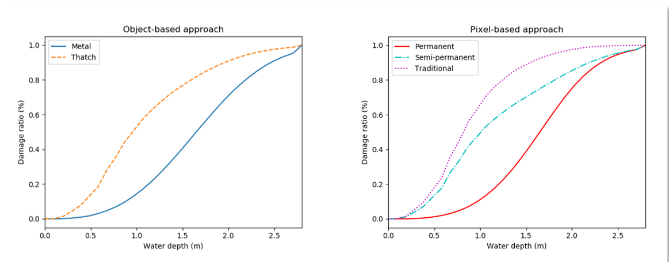
Figure 9: constructed damage curves for the two types derived from field and aerial observation (left-hand panel), and three types derived from the description of building stock at district level (right-hand panel) (Malawi National Statistical Office, 2017). The water depth is the flood water relative to the ground floor.
