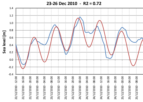
852 Figure A2. Comparison of the observed sea level (in blue) versus the simulated sea level using the harmonic 853 components (in red).
