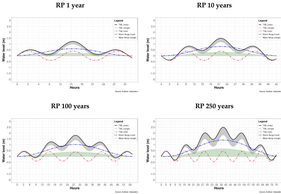
841 Figure A1. Dynamic boundary conditions for simulating theoretical extreme sea level events in ANUGA. The 842 Total Water Level is show as the grey shaded area, while the maximum Total Water Level is shown by the 843 black line, at any given time. The tide (dashed red line), storm surge (dashed blue line) and wave action 844 contribution setup (green shaded area) components define the total water level. Configurations are shown for 845 the return periods of once-in-1, 10, 100 and 250 years.
