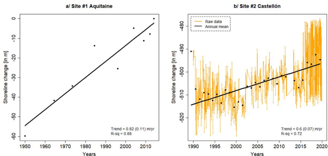
Figure 4: Observed shoreline change evolution in (a) site #1 in Aquitaine and (b) site #2 in Castellón. In Castellón, 859 available observations (orange line) and annual averages (black dots) are shown. The black line shows the linear trends calculated from the annual averages and their standard error are written in brackets. Note that, by convention, positive trends value indicates shoreline retreat.
