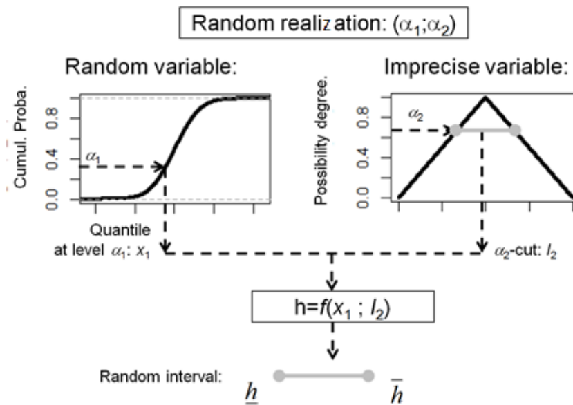
Figure A1. Overview of the main steps for joint propagation of possibility and probability distributions. Adapted from Rohmer and Verdel (2014).
