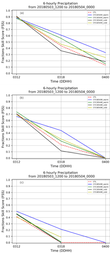
Figure 9: Evolution of FSS calculated in LA region considering the 6-hourly accumulated precipitation for three threshold values: 10 mm 6h -1 (a), 15 mm 6h -1 (b) and 25 mm 6h -1 (c), respectively. Dashed red line represents the CTL, blue line CYC4DVAR_warm, green line CYC3DVAR_warm, black line the CYC3DVAR_cold and yellow line the CYC4DVAR_cold.
