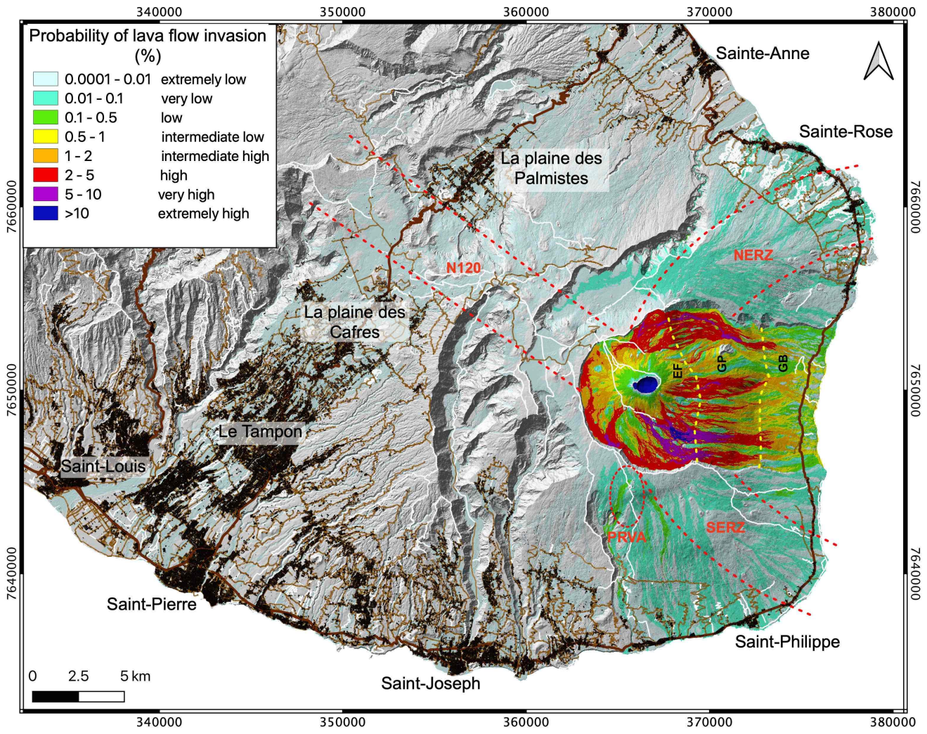
Figure 6: Lava flow hazard map of Piton de la Fournaise. Probability of lava flow invasion is given as percentages and is color coded from extremely low (<0.01 %) to extremely high (>10 %). The buildings are represented as black polygons, and the main roads are in brown (in bold is the RN2 national road) and touristic trails are the white lines (data from from BD TOPO® IGN). The dashed red lines outline the rift zones to the N 120° (N120), to the northeast (NERZ) and to the southeast (SERZ) as well as the Puy Raymond volcanic alignment (PRVA) – (Bachèlery 1981; Michon et al. 2015). The dashed yellow lines separate the Enclos Fouqué caldera (EF) area from the steep slopes “Grandes Pentes” (GP) at 1800-1700 m. a.s.l. and the GP from the eastern lower part “Grand-Brûlé” (GB) at around 500 m. a.s.l. The background is the hill-shade of LiDAR DEM from IGN – released in 2010.
