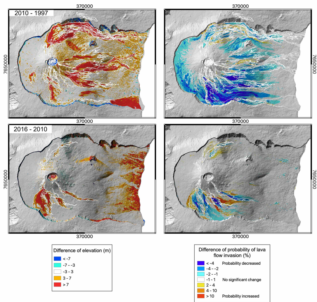
Figure 8: Left column: difference in elevation between 1997 DEM and 2010 DEM (top) and between 2010 DEM and 2016 DEM (bottom). Note that 1) on the 2010-1997 map, the noise in differences is partly due to resolution difference and to slight mis-alignment, 2) on the 2016-2010 map, the positive difference near the coast is due to the vegetation (that has not been removed from the 2016 DEM). Right column: difference of the hazard maps (probability of lava flow invasion in %) built with the data up to 1997 and up to 2010 (top) and built with the data up to 2010 and up to 2016 (bottom).
