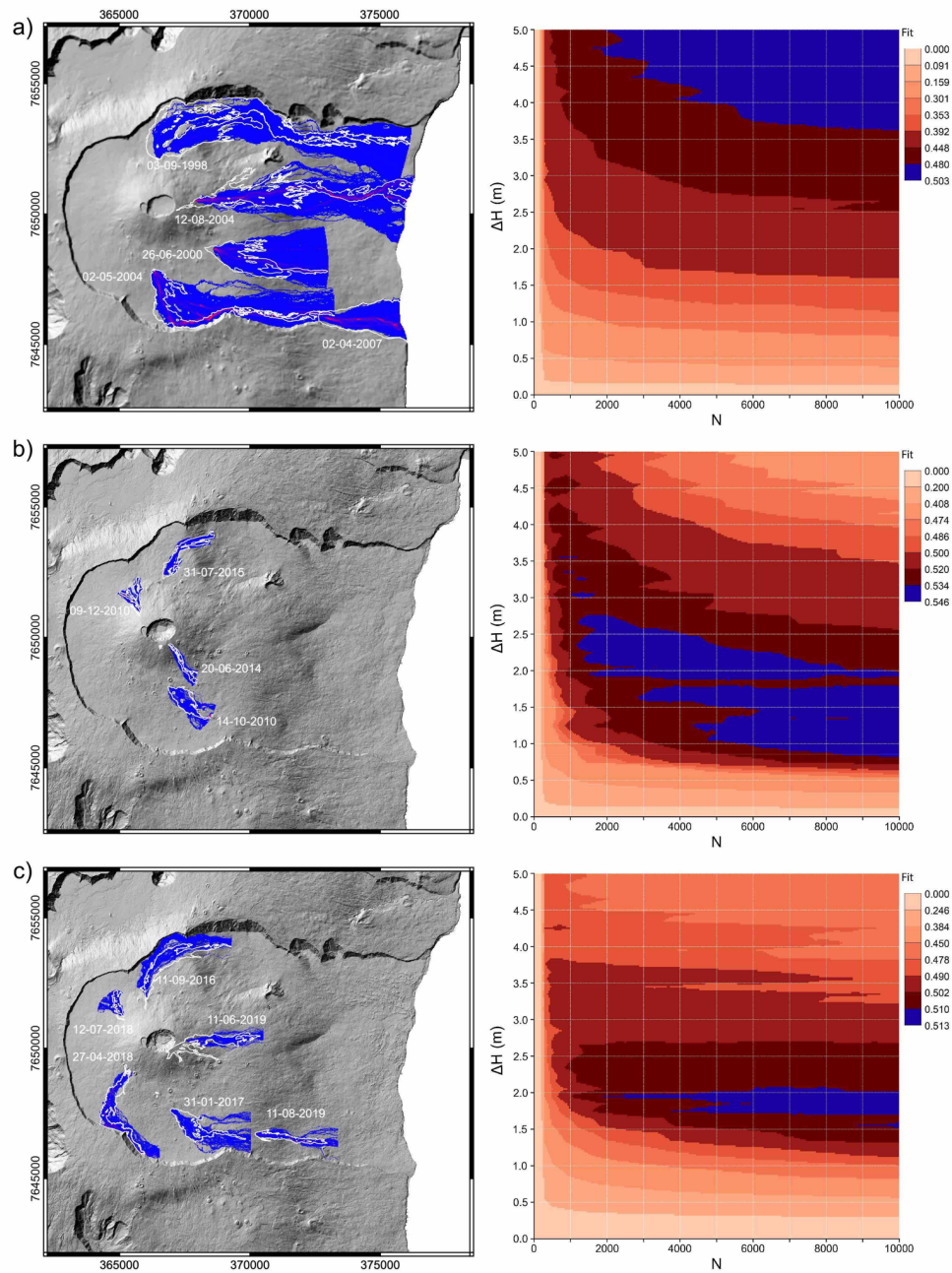
Figure 4: DOWNFLOW calibration for a selected set of lava flows for the three time periods: a) on the 25 m resolution 1997 DEM; b) on the 2010 LiDAR DEM, c) on the 2016 DEM produced from Pleiades. To the left, the maps show the lava flow contours in white and the best DOWNFLOW simulations in blue. To the right, the best fit distribution over the \Delta h - N space (best-fit parameter range are in dark red and blue).
