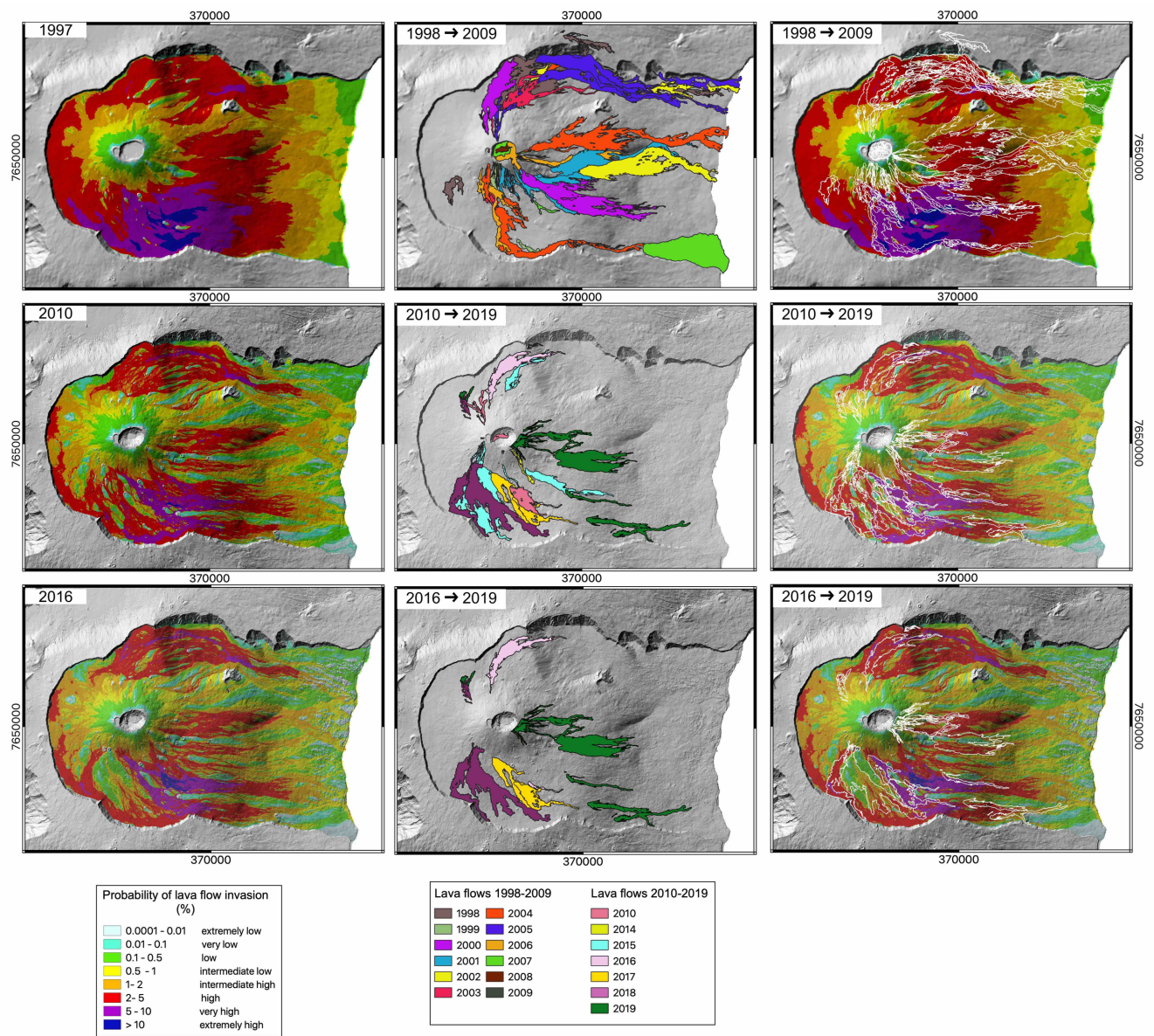
Figure 7: Left column: Evolution of the lava flow hazard maps within the Enclos. The hazard maps are made on the DEM from 1997, 2010 and 2016, respectively, with the corresponding calibration (Fig. 4) and appropriated dataset since 1931 up to the corresponding date (Table 3, Fig. 5). Middle column: successive annual lava flow coverage from the time of the DEM acquisition up to end of 2009 for the 1997 map and up to the end of 2019 for the 2010 and 2016 maps. Right column: maps show the successive lava flows outline (as shown in the middle column) for the given time period.
